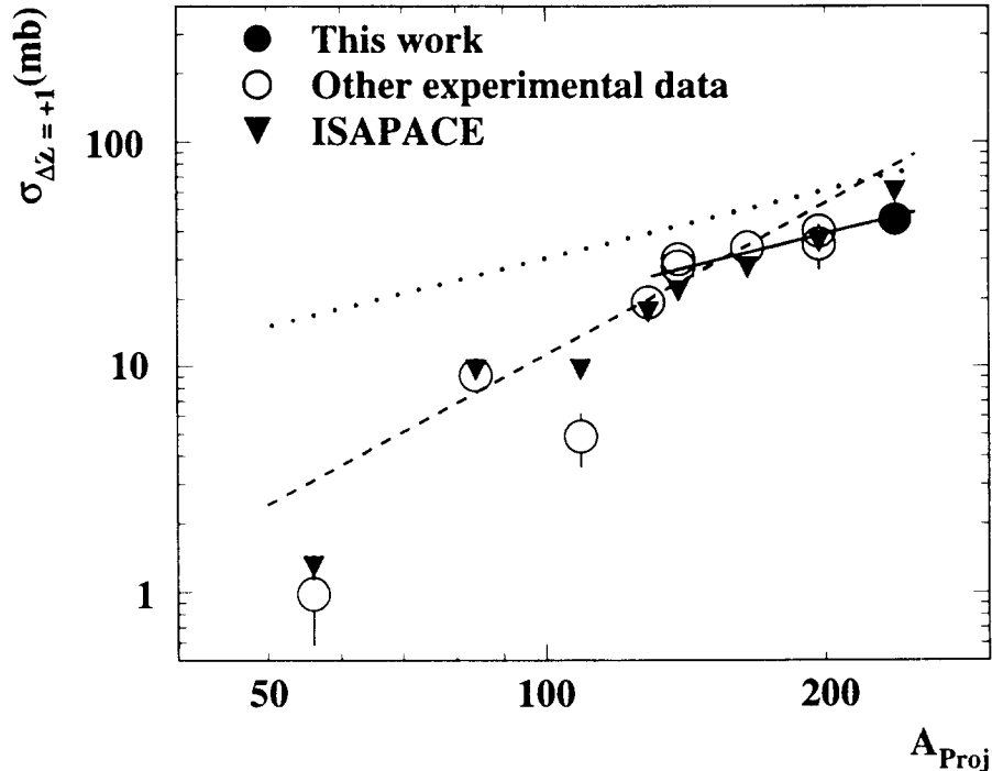
FIG. 4. Experimental cross sections for charge-pickup as a function of the projectile mass from several measurements [2,6,8,22,23]. All data have been obtained by using an Al-target. Both quadratic ( dashed ) and linear ( full line ) dependences are shown. For comparison the results of ISAPACE calculations are shown ( triangles ). The dotted line shows the results from ISABEL calculations, prior to evaporation.
