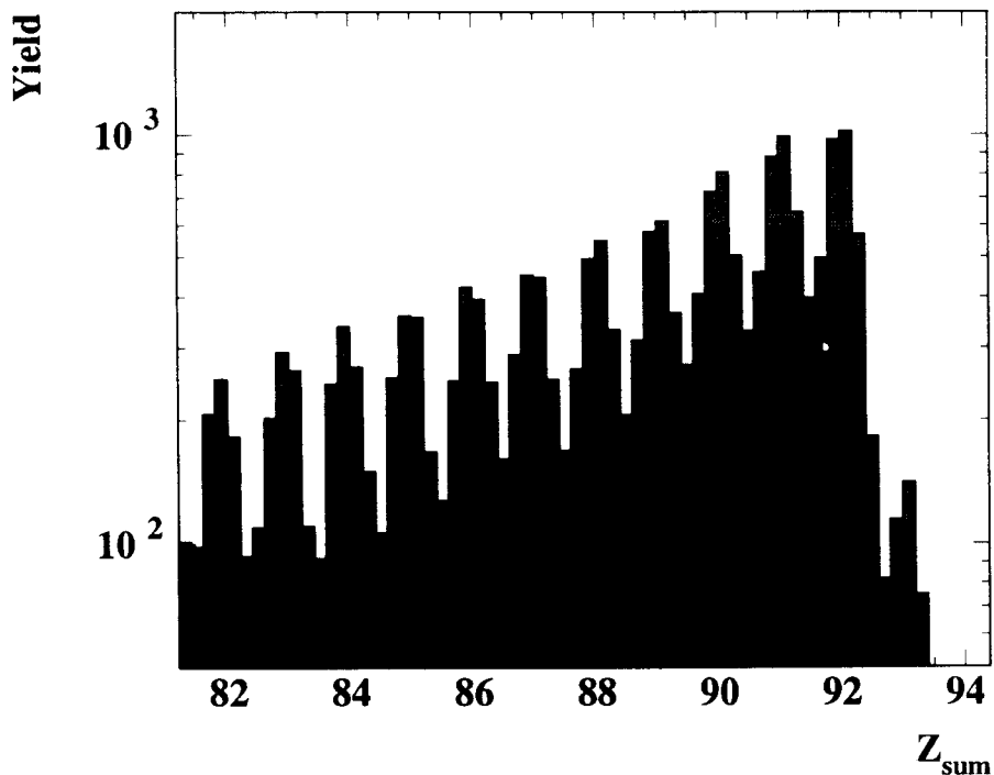
FIG. 1. Spectrum of the sum charge Z_{sum} of fission fragments from the reactions ^{238}\text{U} on Al at E/A = 1000 MeV.
