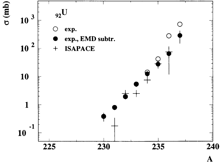
FIG. 3. Experimental cross sections for the production of uranium isotopes in the reaction ^{238}\text{U} + {}^{nat}\text{Cu} at E/A = 950 MeV (open circles, data from Ref. [20]). The nuclear part of the cross sections (full circles, obtained by subtracting the electromagnetic contribution) is compared to the results of ISAPACE calculations (crosses).
