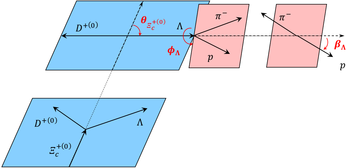
Figure 5: Definition of the three angular variables \cos \theta_{\Xi_c} , \phi_{\Lambda} and \cos \beta_{\Lambda} . The variable \theta_{\Xi_c} is the angle between the \Lambda momentum in the rest frame of the D\Lambda system (denoted as \Xi_c ) and the \Xi_c momentum in the \Xi_b^0 rest frame, referred as the \Xi_c helicity angle. The \Lambda helicity angle \beta_{\Lambda} is the angle between the p momentum in the \Lambda rest frame and the \Lambda momentum in the \Xi_c rest frame. The variable \phi_{\Lambda} is the angle between the \Xi_c \rightarrow D\Lambda and \Lambda \rightarrow p\pi^- decay planes.
