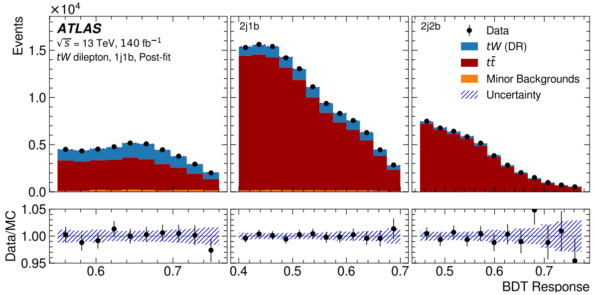
Figure 5: The post-fit BDT response distributions for the three regions used in the fit, after applying the additional BDT selection criteria shown in Figure 3. The uncertainty bands represent both statistical and systematic uncertainties, with each source of systematic uncertainty taking into account correlations with other sources.
