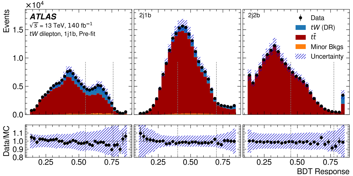
Figure 3: The pre-fit BDT response distributions for the three regions used in the fit. The BDT range used in the fit described in Section 7 is indicated by vertical dashed lines. The first and last bins include the underflow and overflow, respectively. The uncertainty bands represent both statistical and systematic uncertainties, where all sources of systematic uncertainty are assumed to be uncorrelated.
