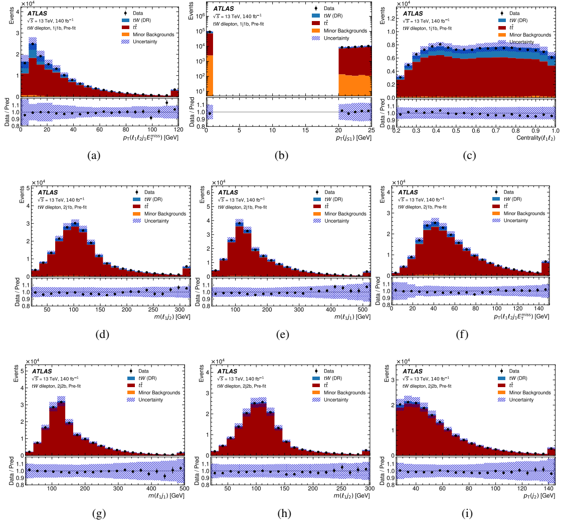
Figure 2: BDT input distributions for the three highest ranked variables (defined in Table 4) from the 1j1b region ((a)–(c)), the 2j1b region ((d)–(f)), and the 2j2b region ((g)–(i)) before the fit. The “minor background” includes Z+jets, diboson, and misidentified/non-prompt lepton contributions. The first and last bin include the underflow and overflow, respectively. The upper panels give the yields in number of events per bin, while the lower panels give the ratios of the numbers of observed events to the total prediction in each bin. The uncertainty bands represent both statistical and systematic uncertainties, where all sources of systematic uncertainty are assumed to be uncorrelated.
