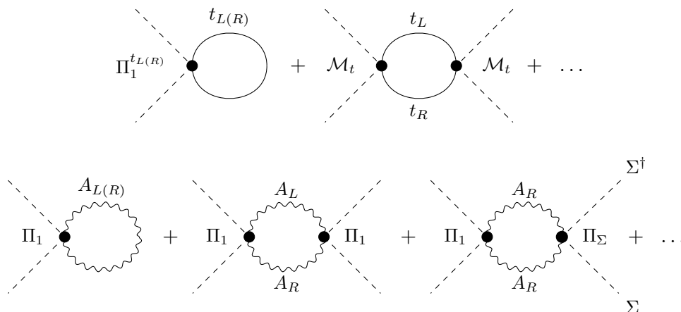
Figure 3. Schematic illustration of the one-loop contributions to the Higgs potential, coming from the explicit Sp(4) breaking required in both the fermion (3.2.2) and gauge (3.3.2) sectors.
