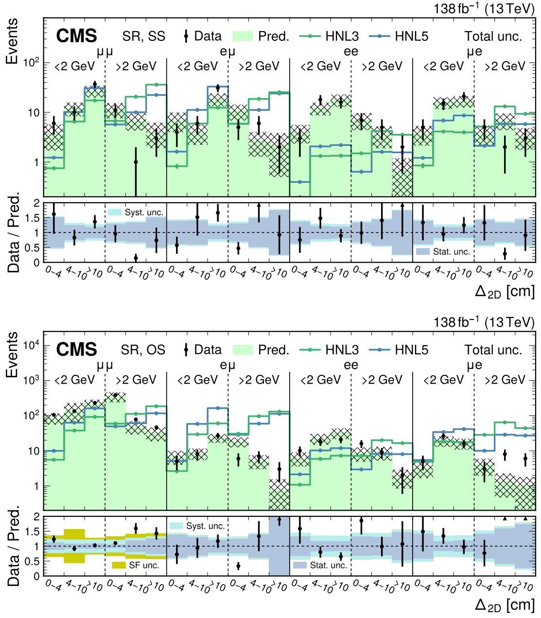
Figure 11. Predicted and observed SR event yields for the SS (upper) and OS (lower) categories of the low-mass PFNs, binned by flavor channel, m_{SV} (as specified below the flavor channel), and \Delta_{2D} . The hashed band represents the total systematic and statistical uncertainty in the background prediction. Signal predictions are shown for two HNL production hypotheses, with m_N = 3 GeV and |V_{\ell N}|^2 = 9.9 \times 10^{-5} (HNL3), and m_N = 5 GeV and |V_{\ell N}|^2 = 1.6 \times 10^{-6} (HNL5). The lower panels show the data-to-prediction ratio and the background prediction uncertainty is split into statistical (“stat.”), systematic (“syst.”), and DY scale factor (“SF”) contributions.
