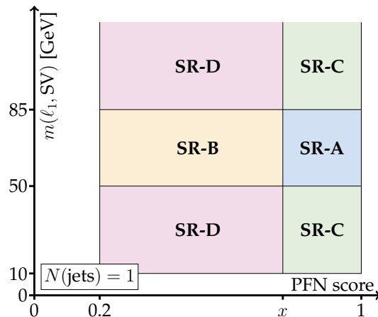
Figure 7. Illustration of the target and sideband region definitions for the ABCD method applied to the SR, in terms of N(\text{jets}) , m(\ell_1, \text{SV}) , and the PFN score.
