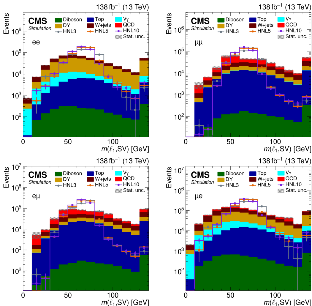
Figure 4. The m(\ell_1, SV) distribution of predicted event yields after applying the selection summarized in table 1, for the ee (upper left), \mu\mu (upper right), e\mu (lower left), and \mu e (lower right) categories. The filled histograms display the predicted background yields. The lines show the predicted yields for three HNL signal scenarios, with m_N = 3 GeV and |V_{\ell N}|^2 = 9.9 \times 10^{-5} (HNL3), m_N = 5 GeV and |V_{\ell N}|^2 = 1.6 \times 10^{-5} (HNL5), and m_N = 10 GeV and |V_{\ell N}|^2 = 5.7 \times 10^{-7} (HNL10). The HNL signal yield is normalized to the total background yield. The last bins include the overflow.
