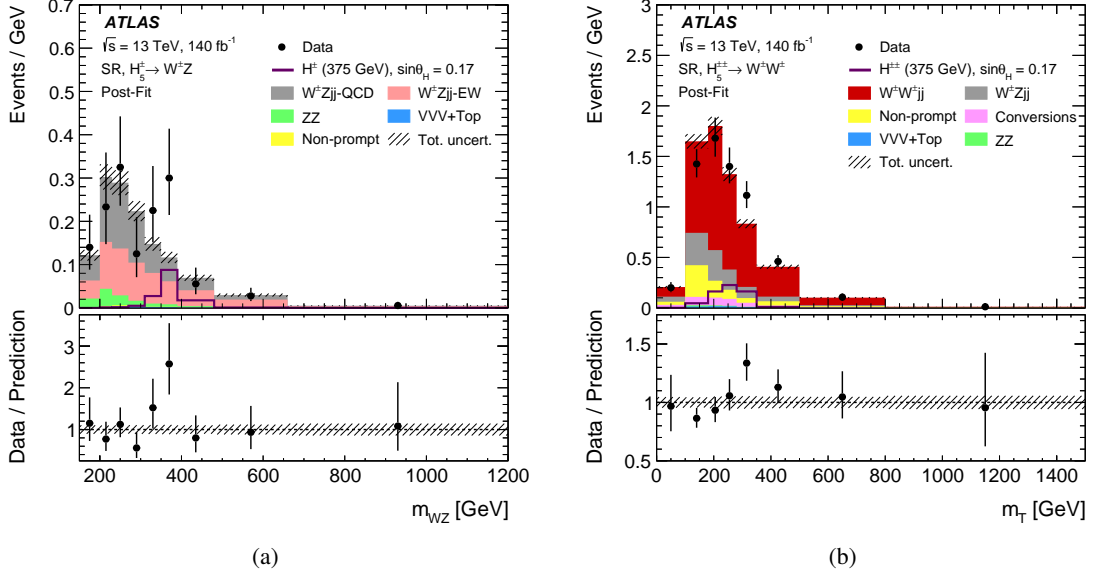
Figure 4: The (a) m_{WZ} and (b) inclusive m_T distributions in the signal regions for the SM background-only hypothesis. Data are shown as black markers with vertical error bars representing the statistical uncertainty. Filled histograms show contributions of various SM processes, with the hatched band representing the total uncertainty. The predicted yields are shown with their best-fit normalisations from the simultaneous fit. The last bin of each distribution includes overflow events. The lower panel shows the ratio of the data to the SM prediction. The line shows the prediction of the GM model for \sin\theta_H = 0.17 and m_{H_5} = 375 GeV, where the \sin\theta_H value corresponds to the expected 95% CL limit for that H_5 mass.
