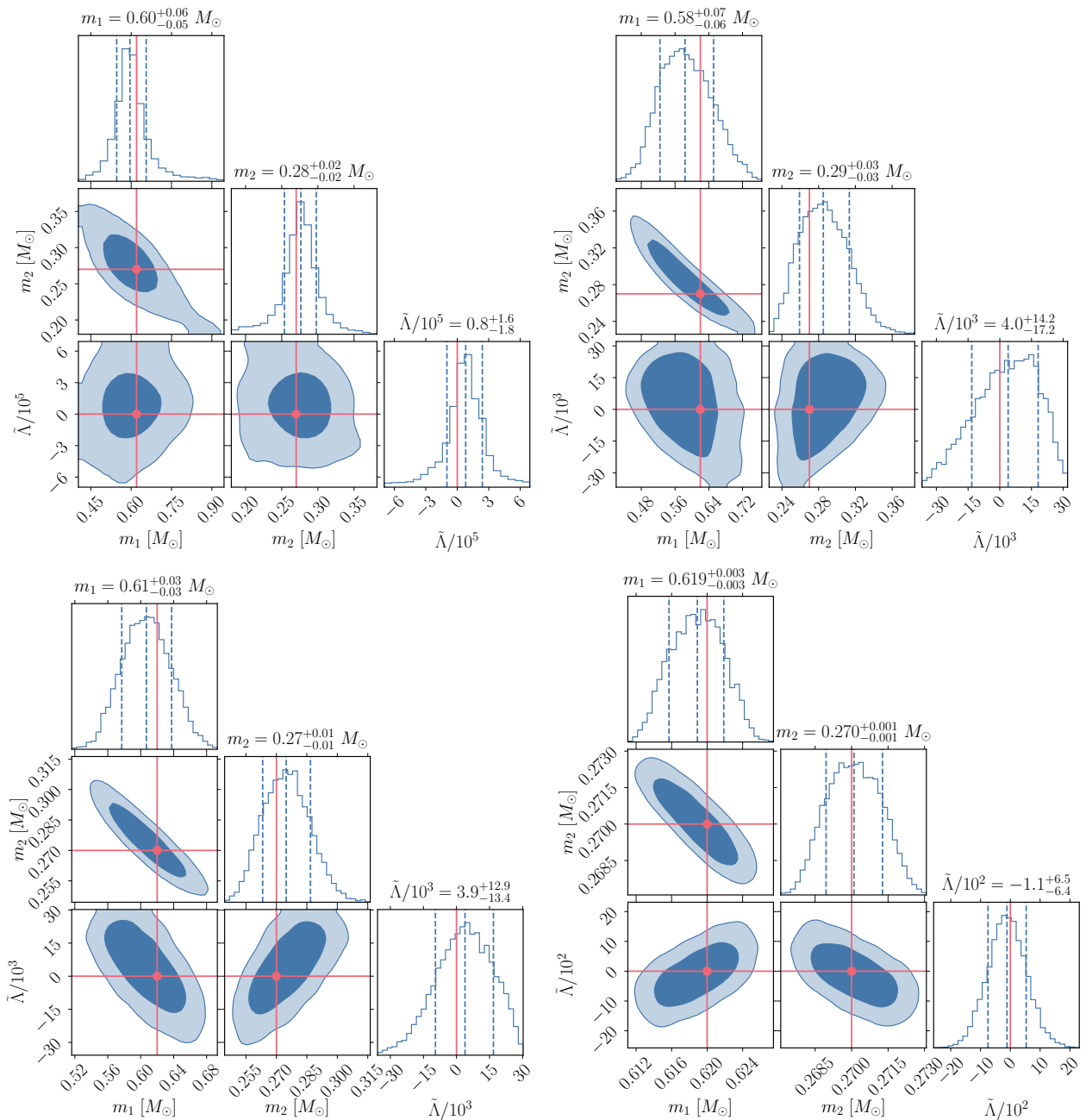
FIG. 3: Posterior distribution of the source frame masses ( m_1, m_2 ) and the \tilde{\Lambda} parameter for respectively O3 (top left), O4 (top right), O5 (bottom left) and ET+2CE (bottom right). The levels of the 2D joint distributions indicate respectively the 68% and 95% credible levels, while the dashed lines on the 1D distributions are the 1\sigma intervals with respect to the median. The orange lines represent the injected values.
