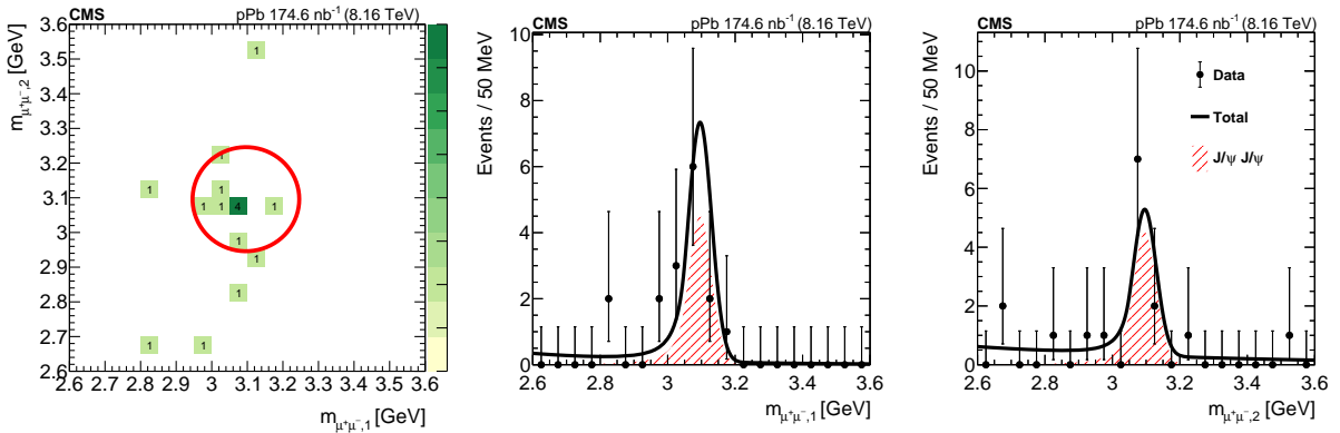
Figure 2: Dimuon invariant mass distributions of the pPb events passing all selection criteria, shown as a 2D map (left panel, with the numbers indicating the counts per bin and the red circle indicating the double J/\psi meson signal region) and its 1D projections for each pair (center and right panels). In the 1D projections, the measured data are represented by the points (with vertical bars showing their Poisson statistical uncertainties), the solid curve shows the overall signal + background fit to the data, and the red hashed area shows the signal yields for the J/\psi J/\psi + X process.
