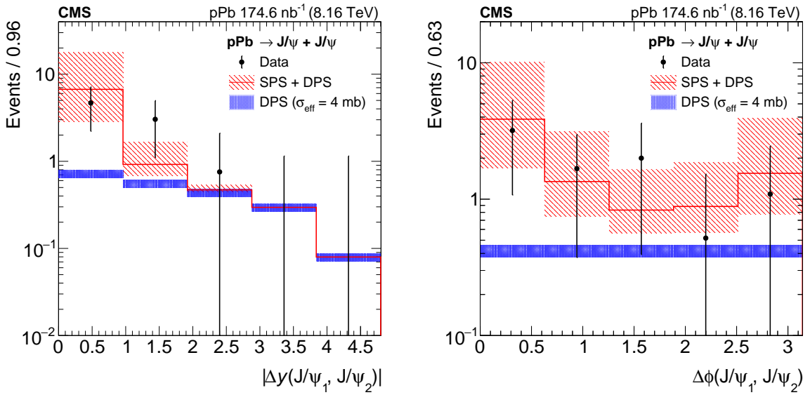
Figure 4: Distribution of rapidity separation (left) between the two J/\psi mesons in data (black markers), fitted template of the expected DPS contribution (blue histogram) normalized to the data outside of the SPS-dominated region (as described in the text), and fitted SPS + DPS distribution (red histogram). Distribution of azimuthal separation (right) between the two J/\psi mesons measured in data (black markers) and expected DPS contribution (blue histogram), and SPS + DPS sum (red histogram), with the relative normalization derived from the \Delta y distribution (left panel), as explained in the text.
