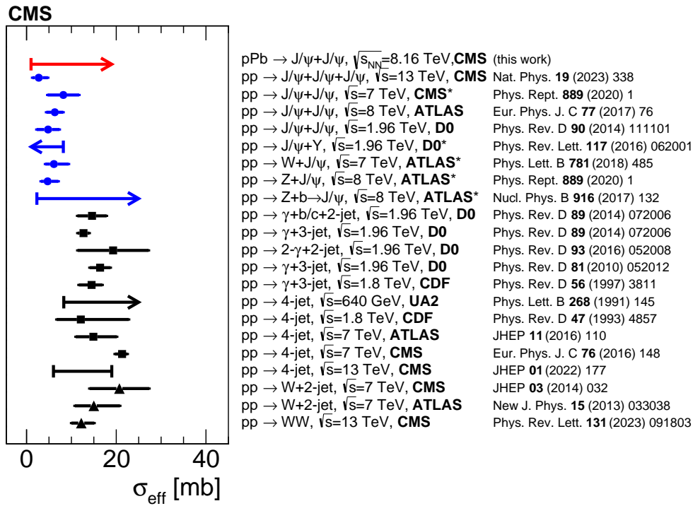
Figure 5: Comparison of the effective DPS cross sections \sigma_{\text{eff}} extracted in this work (red arrow lower limit) with the same parameter derived in pp measurements of double- and triple-quarkonium production [12, 14–16, 37, 77, 79, 80] (blue circles), as well as in final states with jets [81, 82, 85], \gamma + jets [83, 84, 86], W+ jets [19, 20], and double W bosons [26] (black squares). The asterisk shown in a few legend entries indicates that the result has been obtained by more recent phenomenological analyses of the experimental data.
