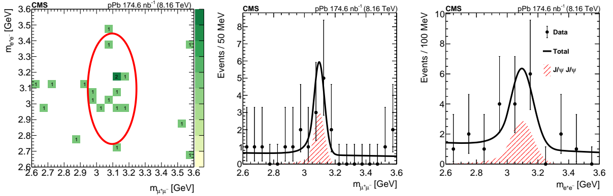
Figure 3: Dilepton invariant mass distributions of the pPb events passing all selection criteria, shown as a 2D map (left panel, with the numbers indicating the counts per bin and the red circle indicating the double J/\psi meson signal region) and its 1D projections for each pair (center and right panels). In the 1D projections, the measured data are represented by the points (vertical bars showing their Poisson statistical uncertainties), the solid curve shows the overall signal + background fit to the data, and the red hashed area shows the signal yields for the J/\psi J/\psi + X process.
