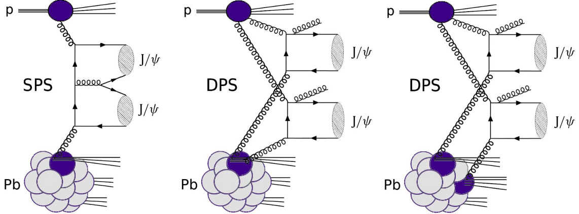
Figure 1: Representative diagrams of SPS (left) and DPS (center and right) contributions to the production of two J/\psi mesons in pPb collisions.
