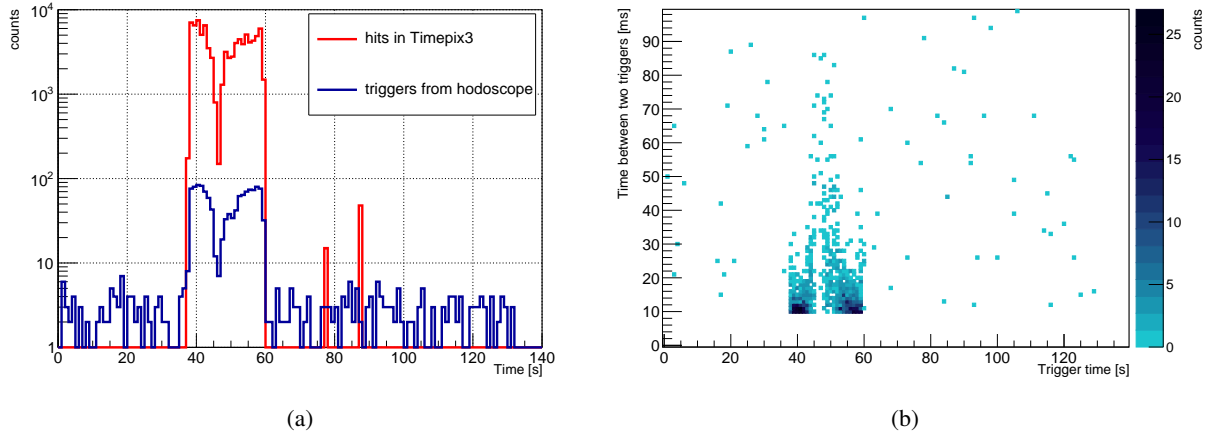
Fig. 4: a) A sample time distribution from one extraction cycle showing the triggers issued by the hodoscope and the number of hits (individual pixels) in the Timepix3. The \sim 20 s long slow extraction of antiprotons is clearly visible (see text for more details). b) The time between two consecutive triggers in ms plotted against the trigger time for the same extraction cycle.
