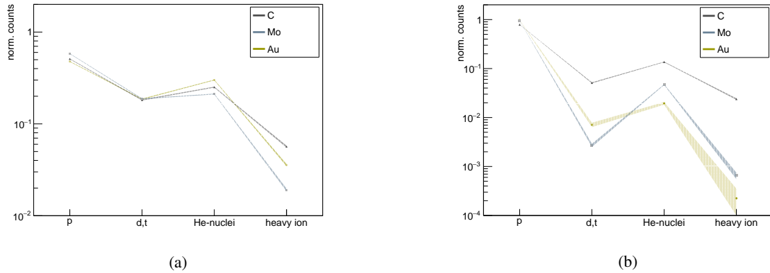
Fig. 15: Breakdown of the different HIPs detected in the Timepix3 for the two models closest to the measured data, a) FLUKA and b) CHIPS. The linear spline is added to guide the eye, but it also displays the associated error values.
