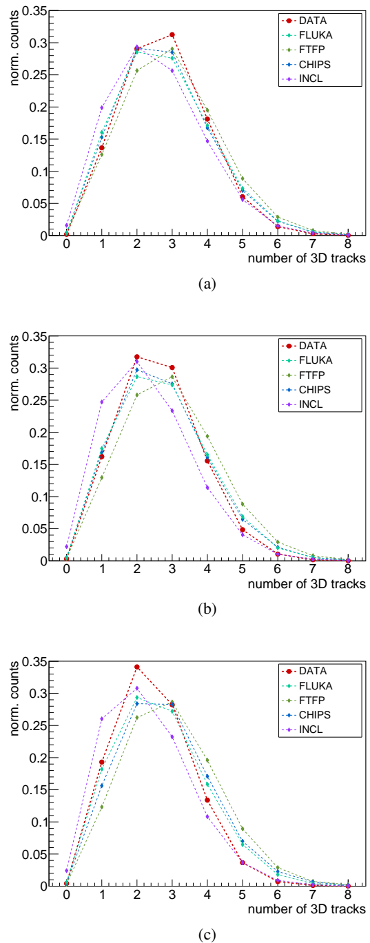
Fig. 12: Multiplicity distributions of MIPs detected by the hodoscope in measured data and Monte Carlo simulations, for antiproton annihilation at rest with a) carbon, b) molybdenum and c) gold.
