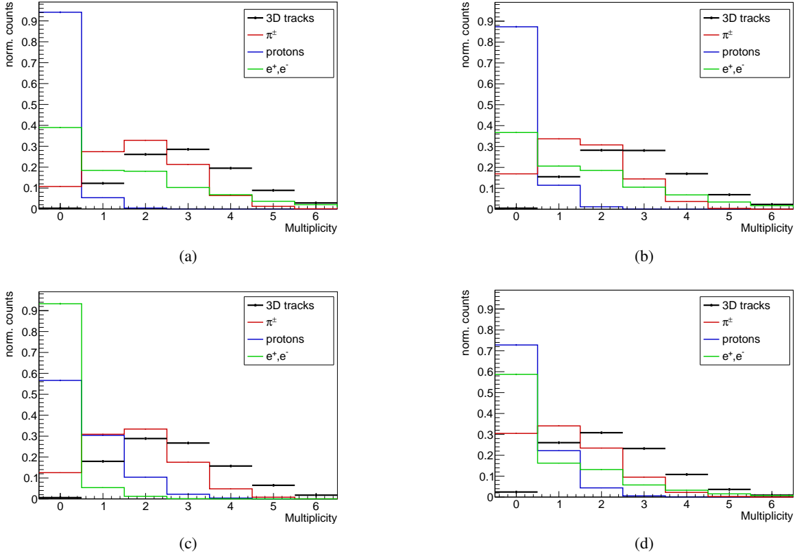
Fig. 9: Multiplicity distributions of 3D reconstructed tracks from MIPs detected by the hodoscope in Monte Carlo simulations, compared to the number of various particles crossing the hodoscope per annihilation event, for antiproton annihilation at rest in gold with a) FTFP, b) CHIPS, c) FLUKA and d) INCL.
