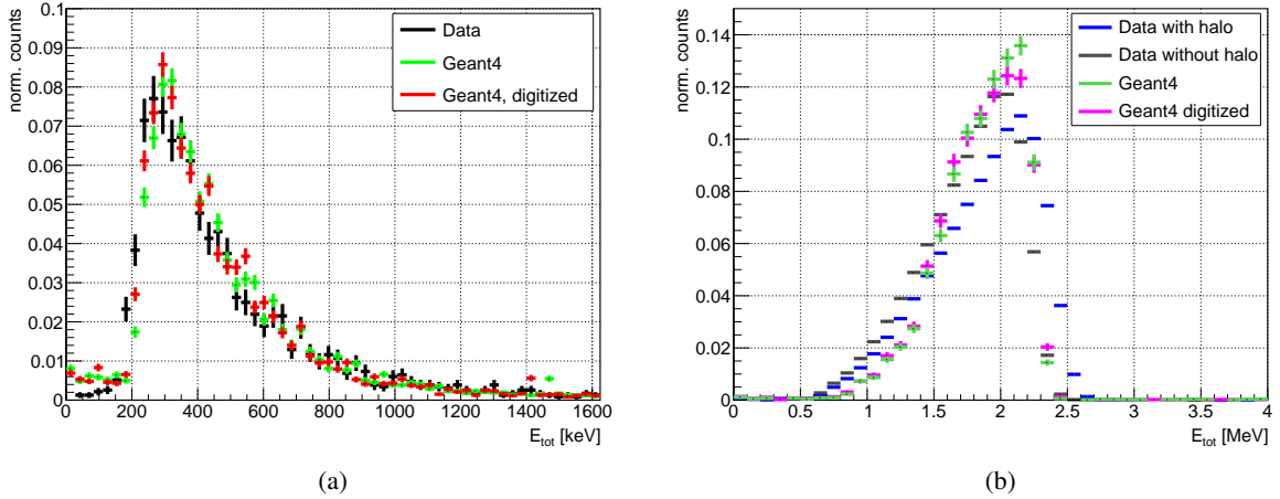
Fig. 10: Comparison between data and Geant4 simulations before and after digitisation for the deposited energy for a) cosmic rays and b) \alpha particles from a ^{241}\text{Am} radioactive source. For the ^{241}\text{Am} the deposited energy before halo removal is also shown for comparison.
