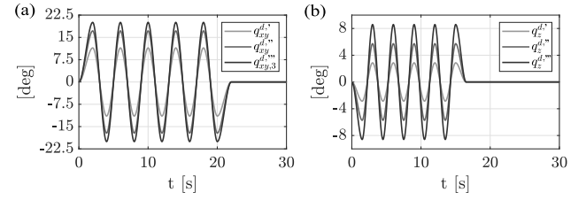
Fig. 7. (a) Sinusoidal joints reference q_{xy}^d for the generation of three oscillations of different amplitudes around x and y axes. The joint reference maximum amplitude has been set to 11.5 deg for the first trajectory q_{xy}^{d'} , to 17 deg for q_{xy}^{d''} and to 20 deg for q_{xy}^{d'''} . (b) Sinusoidal joints reference q_z^d for the generation of three oscillations of different amplitudes around z axis. The joint reference maximum amplitude has been set to 2.85 deg for the first trajectory q_z^{d'} , to 5.7 deg for q_z^{d''} and to 8.6 deg for q_z^{d'''} .
