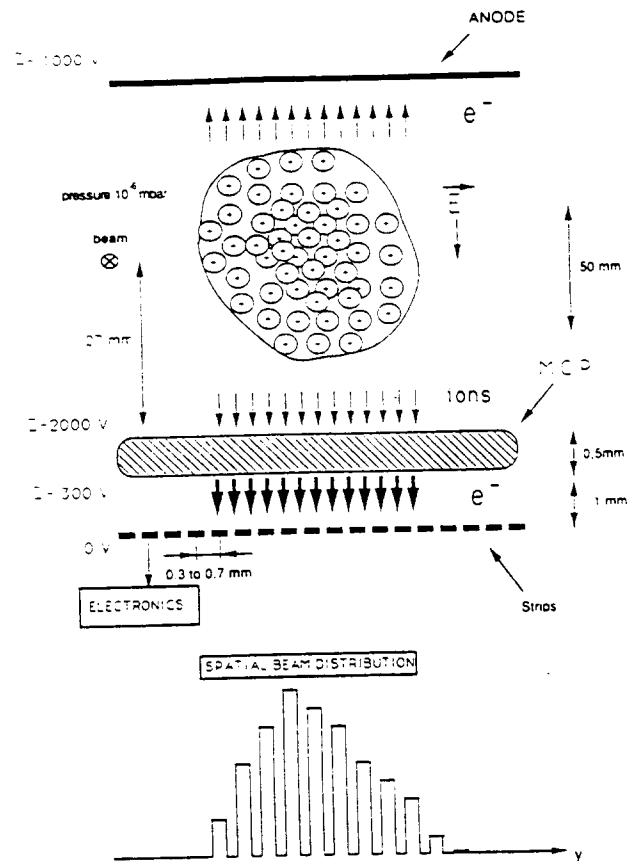
Fig.2. Working principle of the monitor (from ref.[4])
