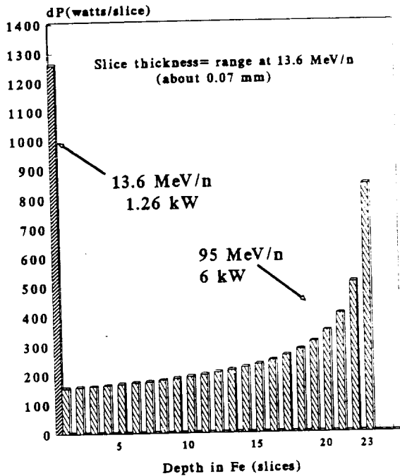
Fig.3. Distribution of the power deposited in Fe by a 1.26 kW, 13.6 MeV/n Ar beam from SSC1 and the corresponding 6 kW, 95 MeV/n beam from SSC2
