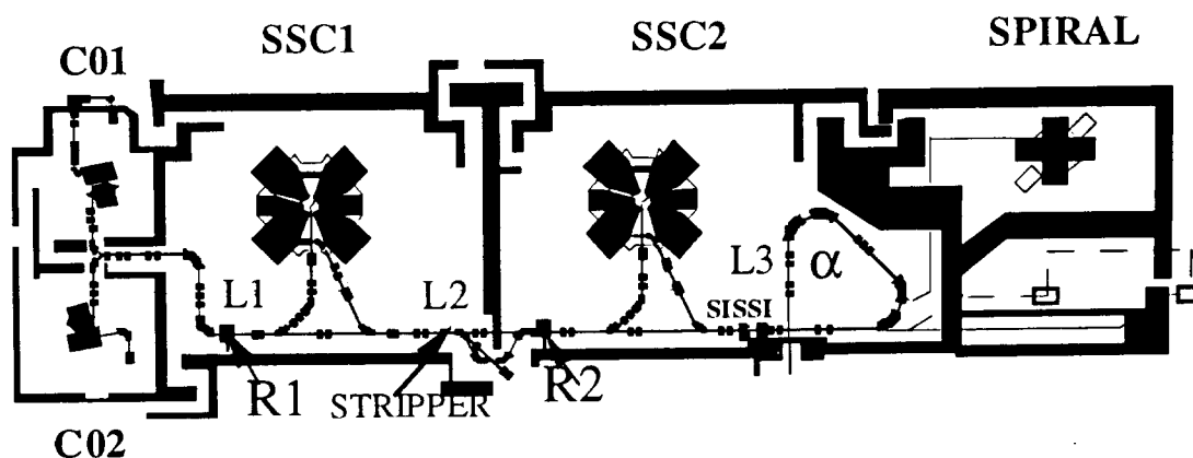
Fig.1. GANIL : general layout . C01, C02 : injector cyclotrons ; SSC1, SSC2 : separated sector cyclotrons ; R1, R2 : rebunchers (the experimental areas are omitted)
