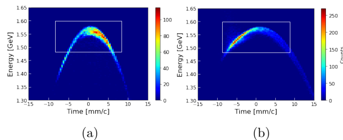
Figure 6: Comparison of the longitudinal phase space of the positrons at the entrance of the DR for two options of the positron linac: based on the LAS structure (a) or the L-band structure (b). The white rectangle represents the energy-time window cut. The reference time is set at 0.
