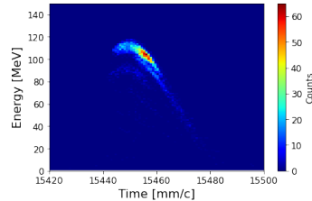
Figure 4: Positron beam longitudinal phase space at the end of the capture section.
