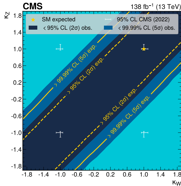
Figure 5: The >95\% ( 2\sigma ) and >99.99\% ( 5\sigma ) exclusion regions in the two-dimensional \kappa_W - \kappa_Z plane are shown by the dark and light blue colors, respectively. Previous CMS measurements of the magnitude of \kappa_W and \kappa_Z at the 95% CL [8] are represented by the horizontal and vertical bars, and the SM expectation is given by the gold star.
