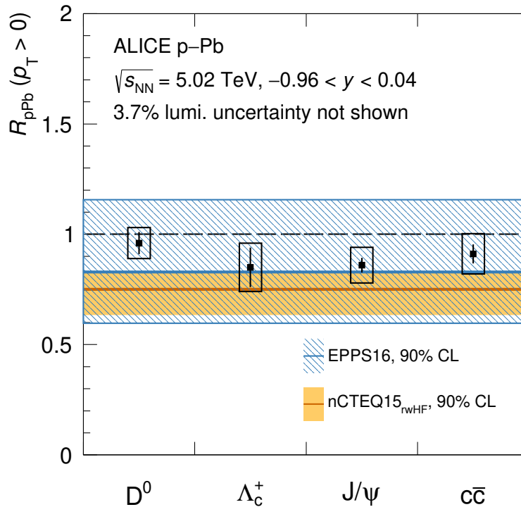
Figure 2: The p_T -integrated nuclear modification factor R_{pPb} for D^0 mesons [21], \Lambda_c^+ baryons [6], J/\psi mesons [31], and c\bar{c} pairs in p–Pb collisions at \sqrt{s_{NN}} = 5.02 TeV. The results are compared with calculations using the nCTEQ15 rWHF [47, 48] (yellow shaded band) and EPPS16 [35] (blue crosshatched band) nPDF sets. The horizontal lines represent the central values of the respective predictions.
