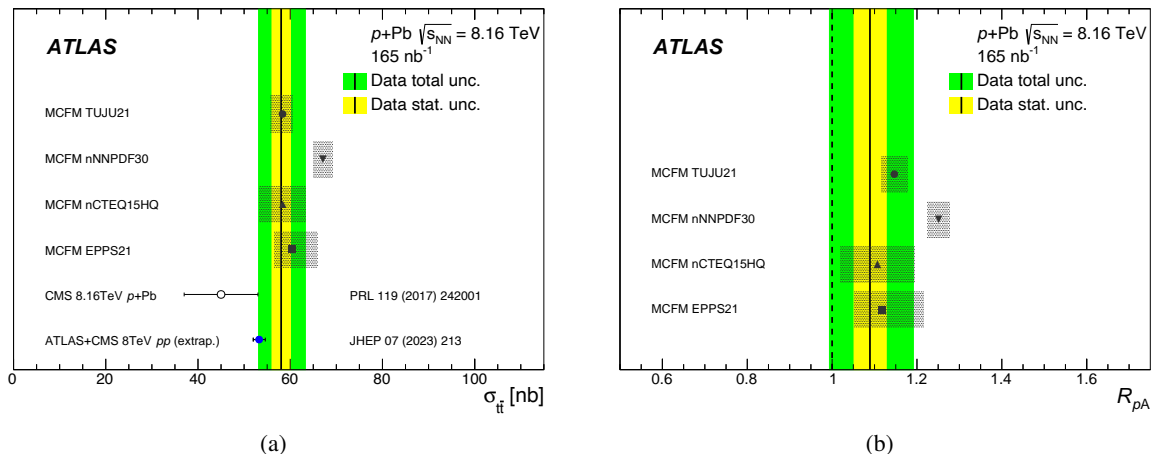
Figure 3: Comparison between measured and predicted values of (a) \sigma_{t\bar{t}} and (b) R_{pA} . \sigma_{t\bar{t}} is also compared with the existing measurement in p +Pb collisions at \sqrt{s_{NN}} = 8.16 TeV [19], and the combined measurement of t\bar{t} production cross-section in pp collisions at \sqrt{s} = 8 TeV from ATLAS and CMS collaborations [68]. The latter is extrapolated to the centre-of-mass energy of this measurement and is using the A_{p_b} factor. Predictions are calculated at NNLO precision using the MCFM code [69] scaled to the p +Pb system and given for different nPDF sets. The uncertainty in the predictions represents the internal PDF uncertainty. The solid black line indicates the measured value. The combined statistical and systematic uncertainty of the measurement is represented by the outer band around the central value, while the statistical component is depicted as the inner band.
