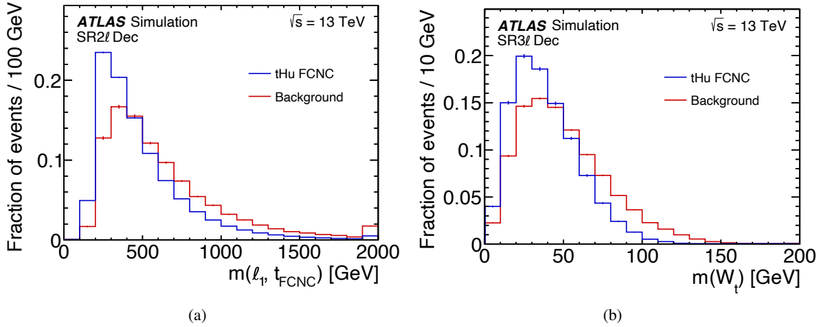
Figure 4: Probability densities of (a) m(\ell_1, t_{\text{FCNC}}) in the SR2 \ell Dec and (b) m(W_t) in the SR3 \ell Dec for the tHu signal process and the sum of all background processes. The vertical lines on bins represent MC-statistical uncertainties. The last bin includes the overflow.
