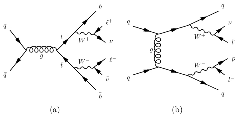
Figure 2. Examples of tree-level Feynman diagrams for the two main backgrounds: (a) t\bar{t} and (b) strong W^+W^-jj .
