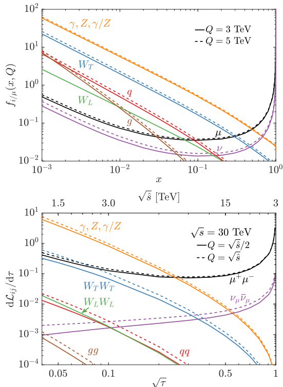
FIG. 2. Distributions for (a) EW PDFs f_i(x) and, (b) parton luminosities d\mathcal{L}_{ij}/d\tau versus \sqrt{\tau} for \sqrt{s} = 30 TeV with a factorization scale Q = \sqrt{\hat{s}}/2 (solid) and \sqrt{\hat{s}} (dashed).
