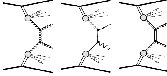
FIG. 19: Inclusive diffractive diagrams. From left to right: jet production and \gamma +jet production in inclusive double Pomeron exchange, as well as jet gap jet events involving double Pomeron exchange
