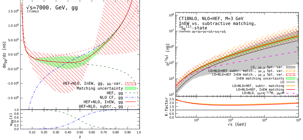
FIG. 7: Left panel: the integrand of the total \eta_c hadro-production cross section as function of z = M^2/\hat{s} in the gg -channel. Dashed line – DL HEF contribution, dash-dotted line – NLO CF contribution, solid line – their matching, according to the Eq. (10), the weight function is shown in the inset. Right panel: The total cross section of hadro-production production of the c\bar{c} [^1S_0^{(1)}] -state as function of \sqrt{s_{pp}} . Plots adopted from the Ref. [186].
