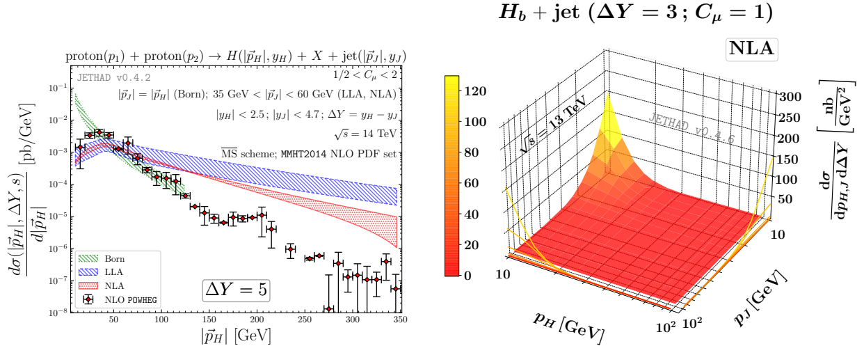
FIG. 4: Left panel: p_T -dependence of the NLA cross section for the inclusive hadroproduction of a Higgs + jet system at \Delta Y = 5 and \sqrt{s} = 14 TeV. Shaded bands give the uncertainty effect of coming from \mu_{R,F} scale variation. Right panel: NLA doubly differential p_T -distribution for the inclusive emission of a H_b + jet system at \Delta Y = 3 and \sqrt{s} = 13 TeV. Calculations are done at natural scales. Figures from Refs. [61, 62].
