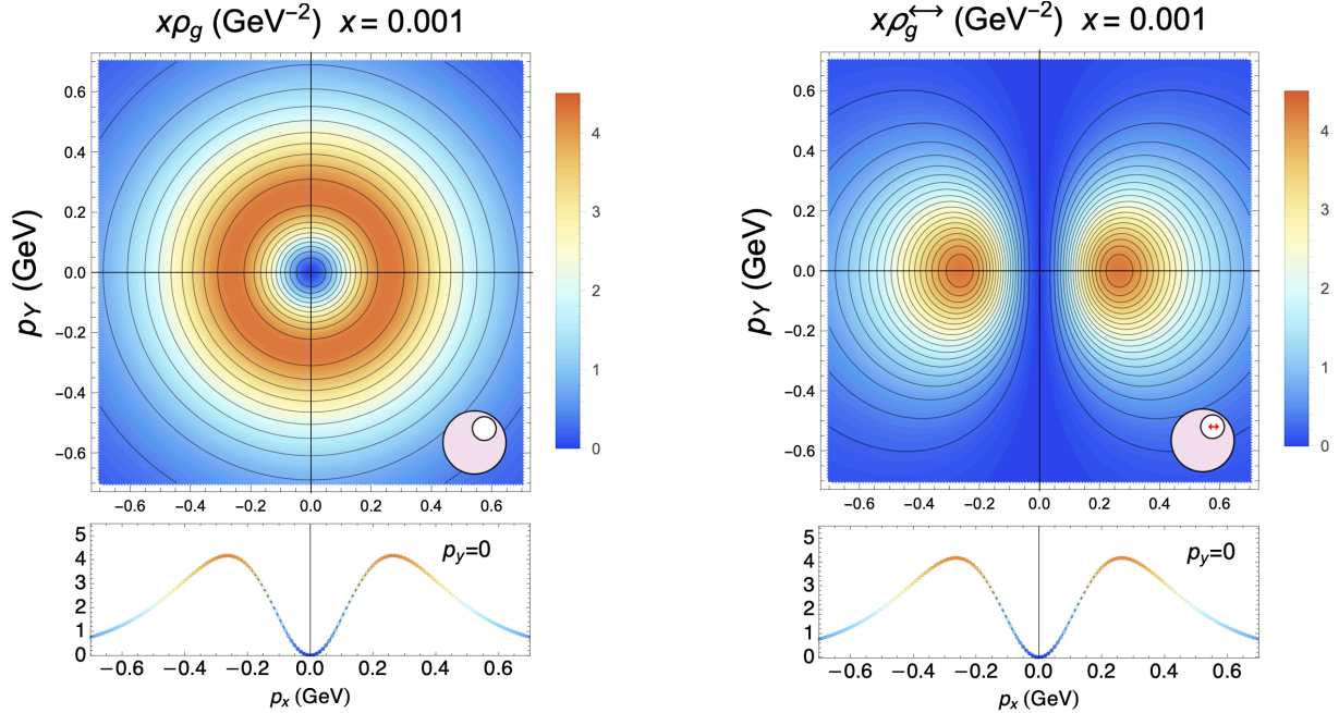
FIG. 9: 3D tomographic imaging of the proton unpolarized (left) and Boer–Mulders (right) gluon TMD densities as functions of the gluon transverse momentum, for x = 10^{-3} and at the initial energy scale, Q_0 = 1.64 GeV. 1D ancillary panels below main contour plots show the density at p_y = 0 . Figures from Ref. [247].
