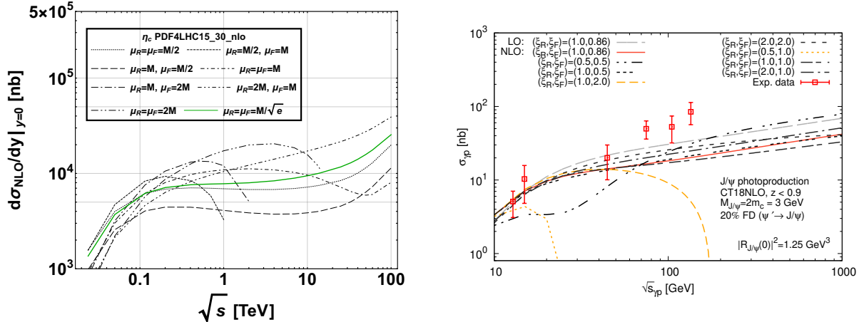
FIG. 6: Collision energy dependence of p_T -integrated prompt inclusive \eta_c hadro-production cross section (left panel, adopted from Ref. [183]) and prompt inclusive J/\psi photoproduction cross section (right panel, adopted from Ref. [184]) at NLO in \alpha_s in the Color-Singlet Model for various choices of factorization ( \mu_F = \xi_F M ) and renormalization ( \mu_R = \xi_R M ) scales.
