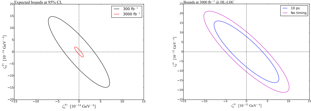
FIG. 24: Expected bounds at 95% CL on the anomalous quartic coupling for 300 \text{ fb}^{-1} and at the HL-LHC with 3000 \text{ fb}^{-1} (no time-of-flight measurement) (left). Expected bounds at 95% CL on the anomalous couplings at the HL-LHC with time-of-flight measurement with precision of 10 ps and without time-of-flight measurement (right). Figure extracted from Ref. [498].
