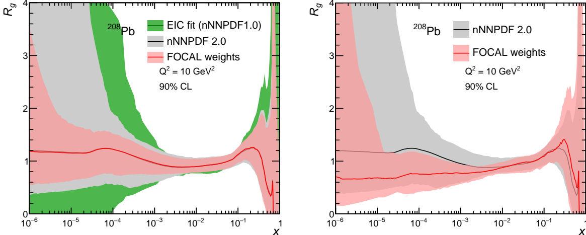
FIG. 13: The nuclear modification of the gluon distribution, R_g , for the Pb nucleus versus x at Q^2 = 10 \text{ GeV}^2/c^2 . (Left) Compared are the nNNPDF2.0 parameterization [303] and fits to the FoCal pseudo-data above 4 \text{ GeV}/c (red band), as well as “high energy” EIC pseudo-data (green band; starting from the nNNPDF1.0 parametrization) [304]. In all cases, 90% confidence-level uncertainty bands are drawn, and the nuclear PDFs are normalized by the proton NNPDF3.1. (Right) Comparison of the original and the reweighted nNNPDF2.0 fits, where the FoCal pseudo-data were shifted by about 0.7 [303].
