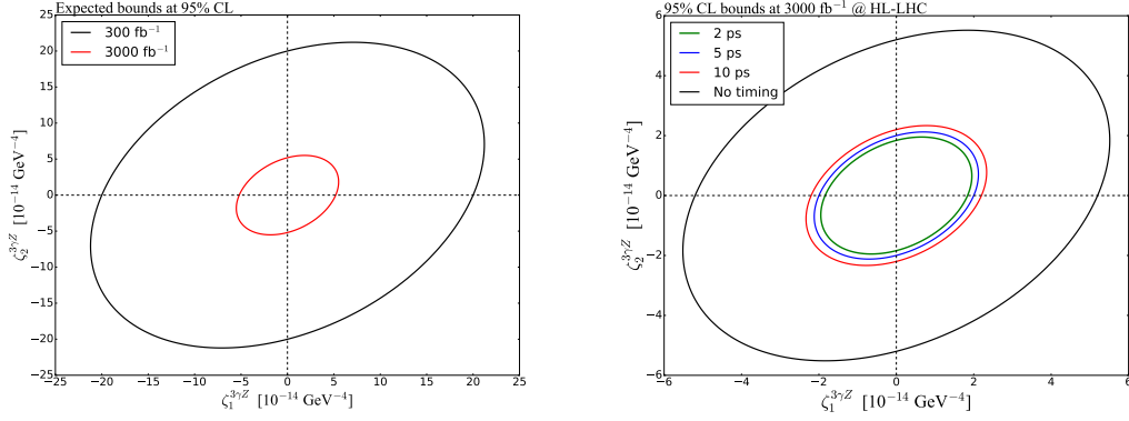
FIG. 25: Expected bounds on the anomalous couplings at 95% CL with 300 \text{ fb}^{-1} and 3000 \text{ fb}^{-1} at the HL-LHC (no time-of-flight measurement) (left). Expected bounds at 95%CL for timing precision of \delta t = 2, 5, 10 \text{ ps} at the HL-LHC (right). Figure extracted from Ref. [498].
