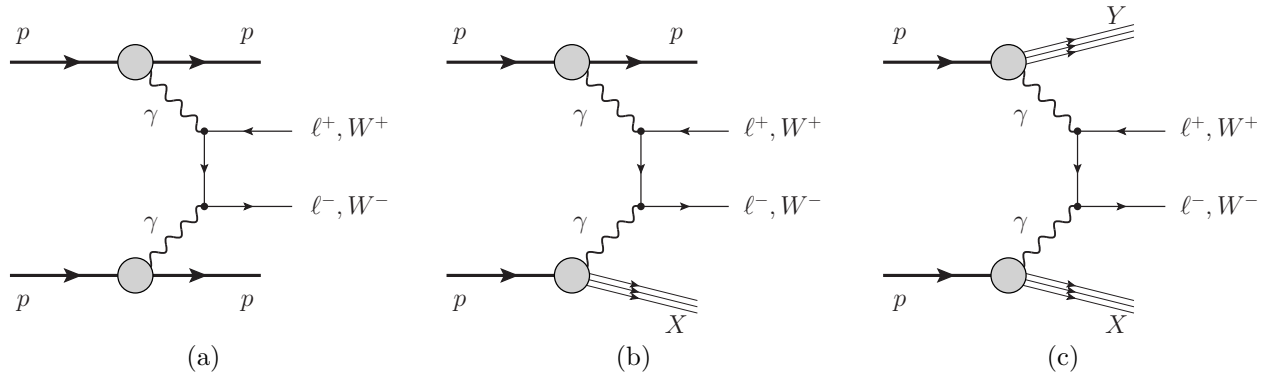
FIG. 21: Processes of particle production in two-photon interactions in hadronic collisions: (a) elastic, (b) semi-elastic, and (c) inelastic case [451].
