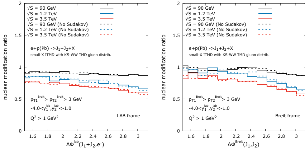
FIG. 11: Nuclear modification factor R_{pA} as a function of the azimuthal angle between the jet system and the scattered electron in LAB frame (left) and as a function of the azimuthal angle between the jets in the Breit frame (right). The calculations are done for three different CM energies per nucleon. Solid lines correspond to calculations using Sudakov form factor and KS-based WW gluon density.
