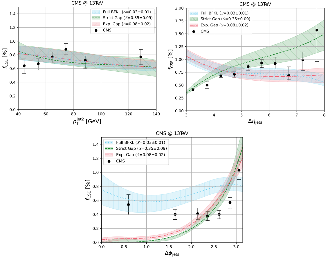
FIG. 8: Measurement of the color-singlet exchange fraction f_{\text{CSE}} at 13 TeV by the CMS Collaboration [193]. Theoretical predictions based on BFKL calculations at next-to-leading logarithmic accuracy assuming experimental gap (“exp gap”), a theoretical-like gap (“strict gap”), and no gap requirement (“full BFKL”) are presented. The bands represent uncertainties related to factorization and renormalization scale variations. The gap survival probabilities, indicated in the legend, were fit with a \chi^2 scan.
