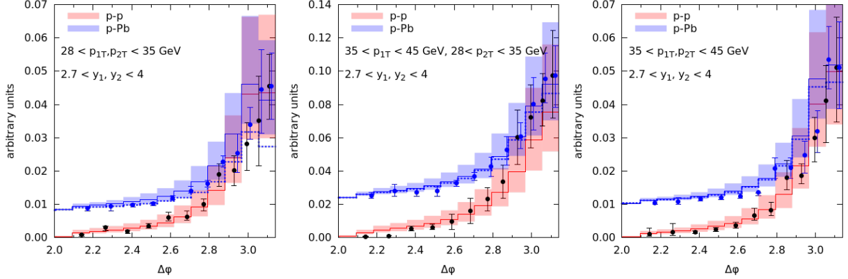
FIG. 10: Broadening of azimuthal decorrelations in p - Pb collisions vs p - p collisions for different sets of cuts imposed on the jets' transverse momenta. The plots show normalized cross sections as functions of the azimuthal distance between the two leading jets, \Delta\phi . The points show the experimental data [280] for p - p and p - Pb , where the p - Pb data were shifted by a pedestal, so that the values in the bin \Delta\phi \sim \pi are the same. Theoretical calculations are represented by the histograms with uncertainty bands coming from varying the scale by factors 1/2 and 2.
