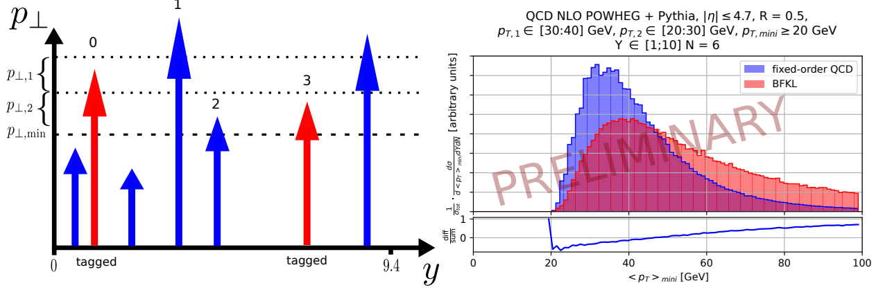
FIG. 2: Left: Minijets below p_{\perp, \text{min}} = 20 GeV are ignored for the calculation of the observables. Right: The observable from Eqs. 2.
