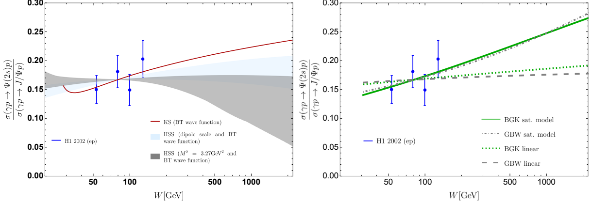
FIG. 16: Energy dependence of the ratio of \Psi(2s) vs. J/\Psi photoproduction cross-section. We further display photoproduction data measured at HERA by the H1 collaboration [388], which we further use to adjust the normalization. Left: Implementation of the KS and HSS gluon distributions for the Buchmüller-Tye (BT) vector meson wave functions, see [166] for details. The shaded regions correspond to a variation of the scale \bar{M} \rightarrow \{\bar{M}/\sqrt{2}, \bar{M}\sqrt{2}\} . Right: Implementation based on BKG and GBW saturation model and their corresponding linearized versions, using numerical values found in [389] from a fit to HERA data.
