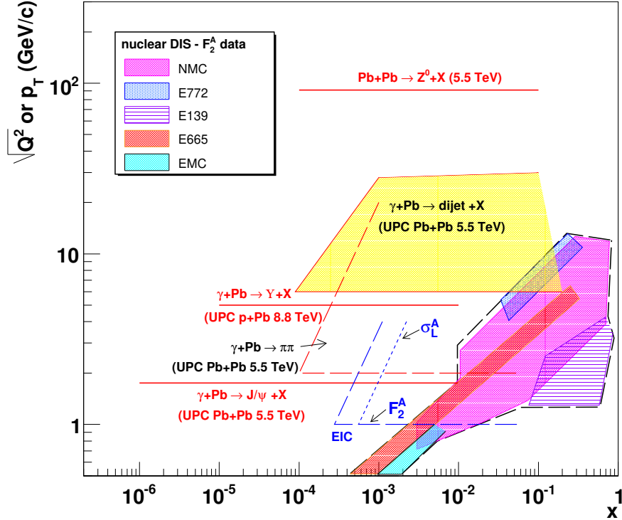
FIG. 15: The kinematic range in which UPCs at the LHC can probe gluons in protons and nuclei in quarkonium production, dijet and di-hadron production. The Q value for typical gluon virtuality in exclusive quarkonium photoproduction is shown for J/\Psi and \Upsilon . The transverse momentum of the jet or leading pion sets the scale for dijet and \pi\pi production respectively. For comparison, the kinematic ranges for J/\Psi at RHIC, F_2^A and \sigma_L^A at eRHIC and Z^0 hadro-production at the LHC are also shown. Figure taken from [317]
