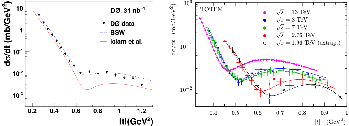
FIG. 17: Left: p\bar{p} elastic cross section as a function of |t| at 1.96 TeV from the D0 collaboration at the Tevatron. Right: pp elastic cross sections as a function of |t| at 2.76, 7, 8, and 13 TeV from the TOTEM collaboration at the LHC (full circles), and extrapolation to the Tevatron center-of-mass energy at 1.96 TeV (empty circles).
