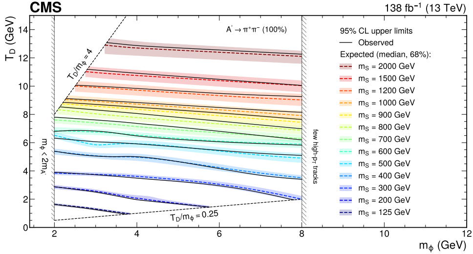
Figure 4: The observed and expected exclusions for the nominal S cross section in the plane of m_\phi and T_D , for various m_S values, for the case m_{A'} = 1.0 GeV ( A' \rightarrow \pi^+\pi^- with \mathcal{B} = 100\% ). The regions below the observed limits are excluded.
