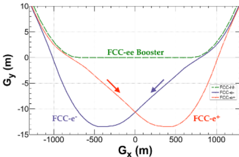
Figure 1. Crab-waist layout of the FCC-ee around the interaction point. Reproduced from [10]. CC BY 4.0.
