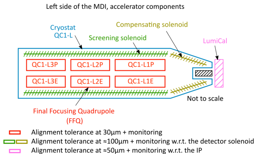
Figure 2. Current design of the FCC-ee MDI, with the inner components locations and initial alignment requirements [12].
