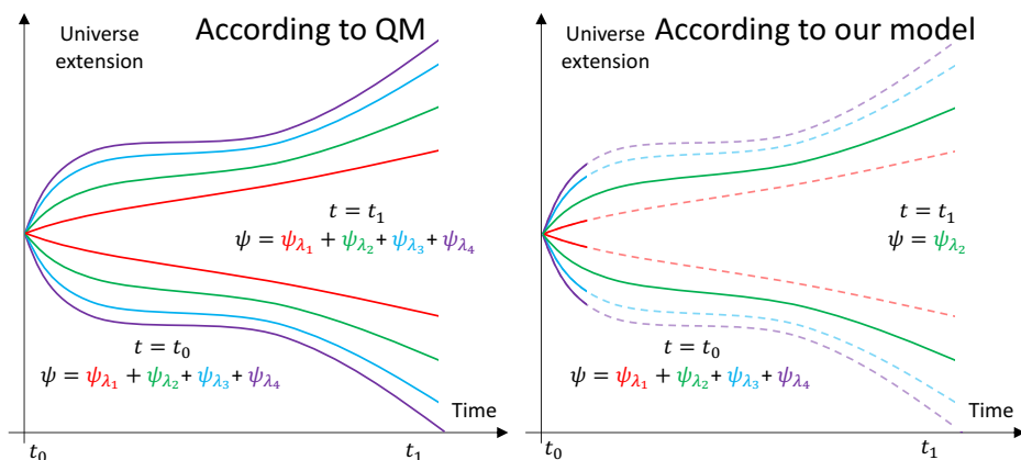
Figure 1. (Left panel) According to quantum mechanics, an initial superposition of the Universe \Psi = \Psi_{\lambda_1} + \Psi_{\lambda_2} + \Psi_{\lambda_3} + \Psi_{\lambda_4} at time t_0 is conserved under the unitary dynamics of the Schrödinger equation. The state of the Universe never collapses in one eigenstate of \hat{\lambda} for any later time t_1 . (Right panel) The introduction of collapse terms in the Wheeler-DeWitt equation allows for the collapse of the wavefunction from the initial superposition at time t_0 into a single eigenstate of \hat{\lambda} (e.g., \Psi = \Psi_{\lambda_2} ) at a time t_1 .
