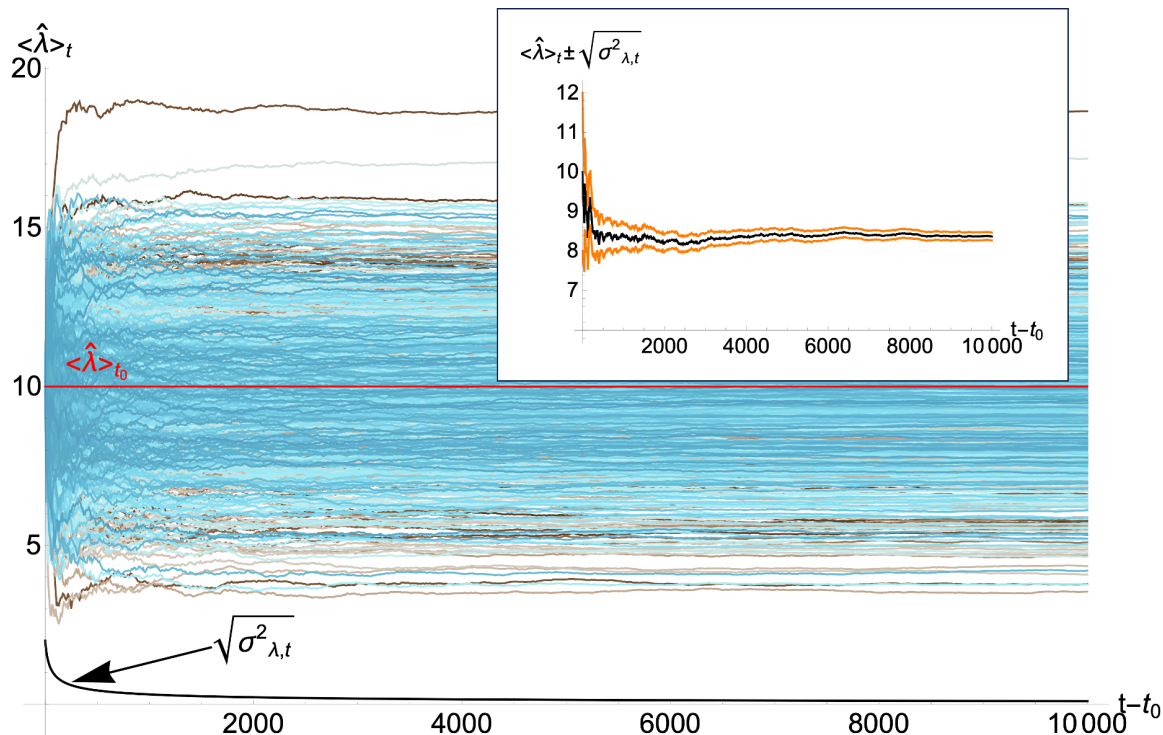
Figure 2. Mean \langle \hat{\lambda} \rangle_t for 1000 different realisations of the noise field W_t , with \epsilon = 0.05 and an initial state with Q(\lambda) \propto e^{-(\lambda-\lambda_0)^2/4\sigma_0^2} with \lambda_0 = 10 and \sigma_0^2 = 4 . The red line highlights the initial value of \langle \hat{\lambda} \rangle_{t_0} , while the black line shows the evolution of \sigma_{\lambda,t} under the Gaussian assumption. The inset show a single realisation of the noise: in black \langle \hat{\lambda} \rangle_t , in orange \langle \hat{\lambda} \rangle_t \pm \sqrt{\sigma^2_{\lambda,t}} .
