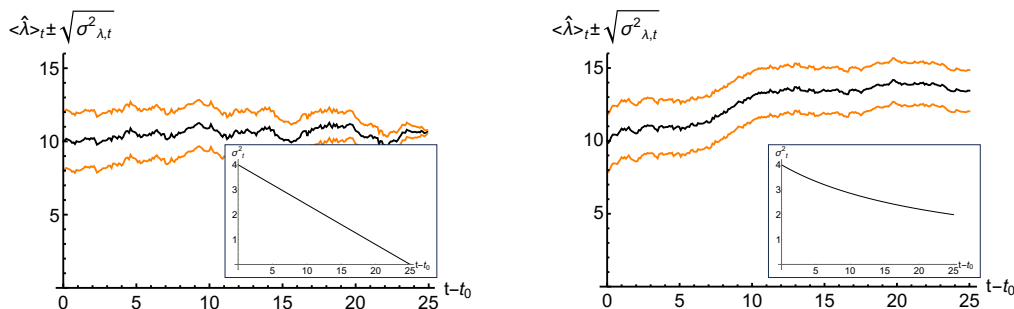
Figure 3. Comparison of the solutions \langle \hat{\lambda} \rangle_t as expressed respectively in eq. (A.14a) and eq. (A.15a). The insets report the corresponding variances \sigma_t^2 [cf. eq. (A.14b) and eq. (A.15b)]. The perturbative solution (left panel) is associated to a fast decaying variance, while the exact solution (right panel) is localised on a much longer time-scale.
