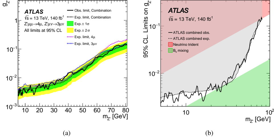
Figure 4: Results from the statistical combination of the 3\mu and 4\mu channels: (a) observed and expected 95% CL upper limits on g as a function of m_{Z'} , (b) exclusion contour of g compared with the limits inferred from the neutrino-trident (red) and the B_s mixing (green) experimental results [21].
