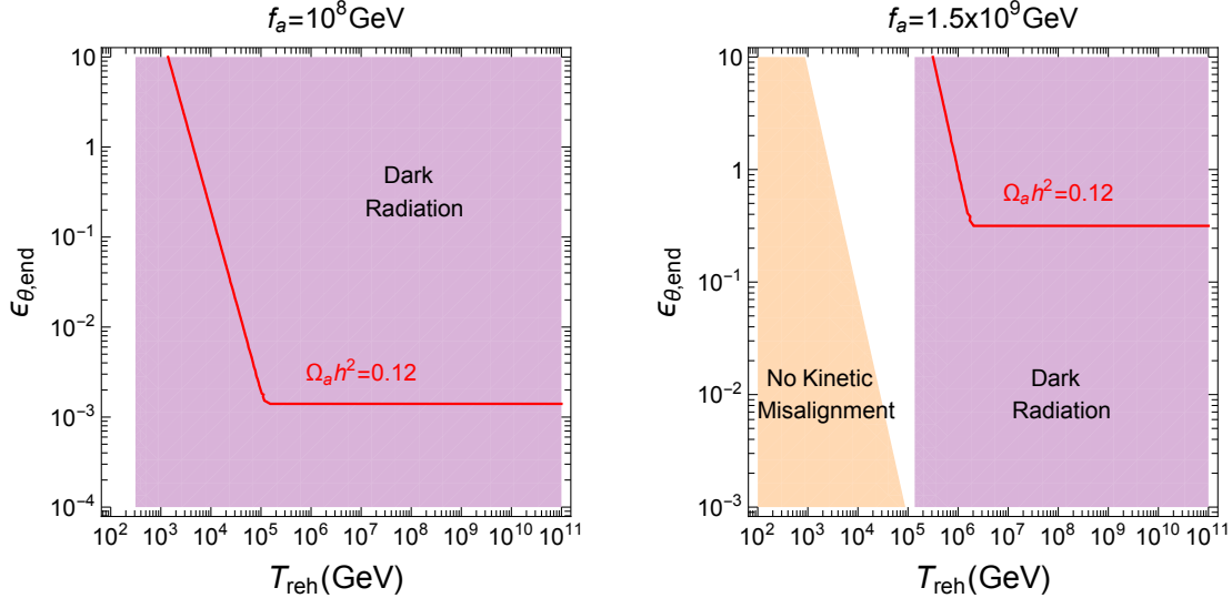
Figure 2: Parameter space in the reheating temperature T_{\text{reh}} vs \epsilon_{\theta, \text{end}} for axion dark matter with kinetic misalignment. The correct relic density is obtained by the axion kinetic misalignment along the red line. The kinetic misalignment is sub-dominant in orange region, and the axions produced from the inflaton scattering were in thermal equilibrium, becoming dark radiation at a detectable level in purple regions. We took f_a = 10^8 GeV, 1, 5 \times 10^9 GeV on the left and right plots, respectively.
