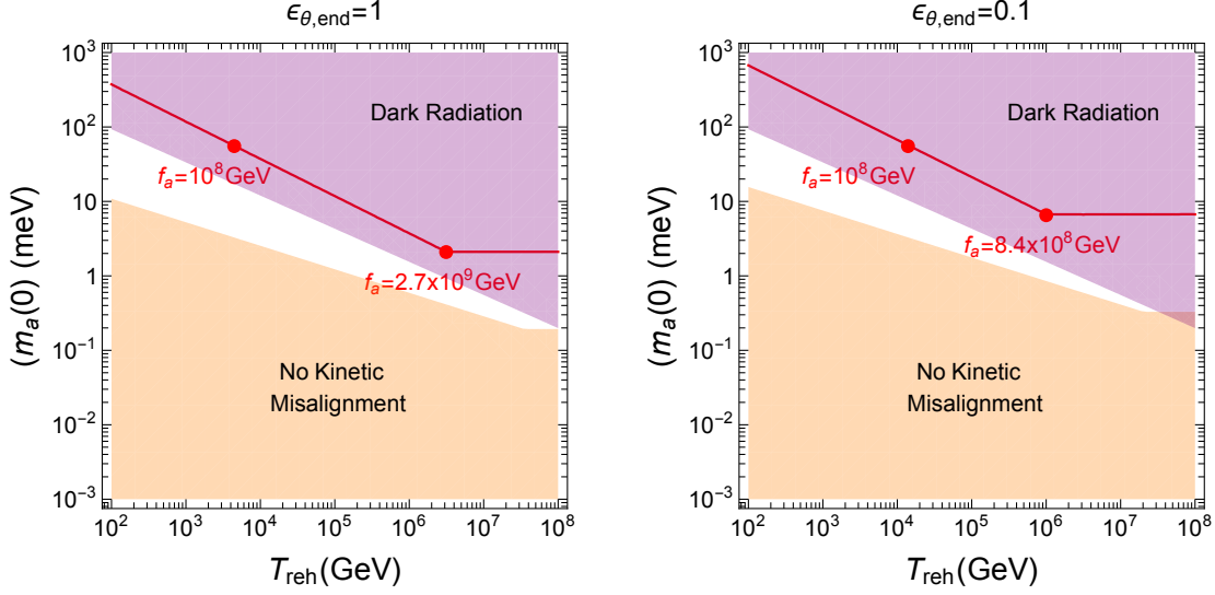
Figure 3: Parameter space in the reheating temperature T_{\text{reh}} vs the axion mass m_a(0) for axion dark matter with kinetic misalignment. The correct relic density is obtained by the axion kinetic misalignment along the red line. The kinetic misalignment is sub-dominant in orange regions and the axions produced from the inflaton scattering were in thermal equilibrium, becoming dark radiation at a detectable level in purple regions. We took \epsilon_{\theta,\text{end}} = 1, 0.1 on the left and right plots, respectively.
