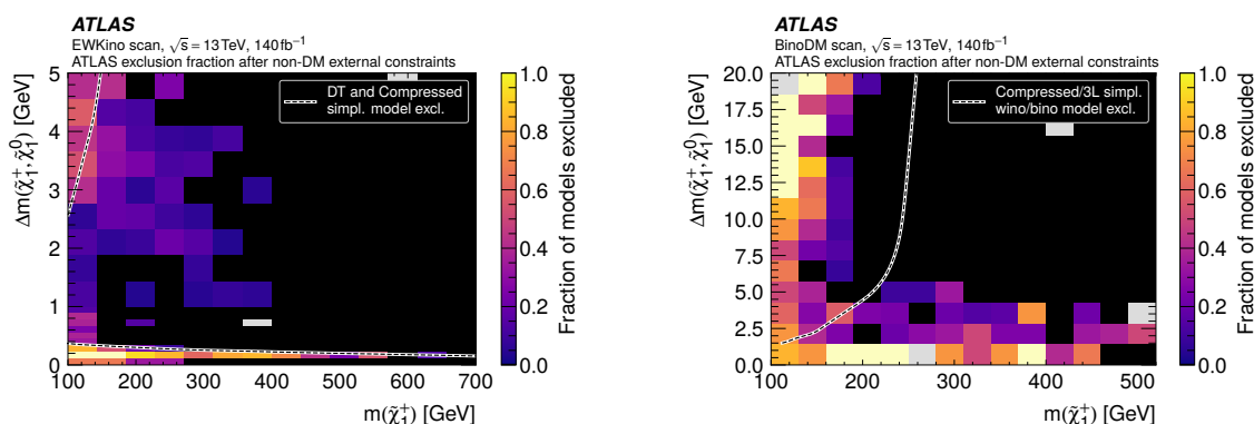
(a) EWKino scan ( \Delta m(\tilde{\chi}_1^\pm, \tilde{\chi}_1^0) < 5 GeV). (b) BinoDM scan ( \Delta m(\tilde{\chi}_1^\pm, \tilde{\chi}_1^0) < 20 GeV).
