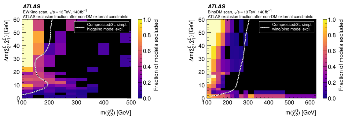
(a) EWKino scan. (b) BinoDM scan.
