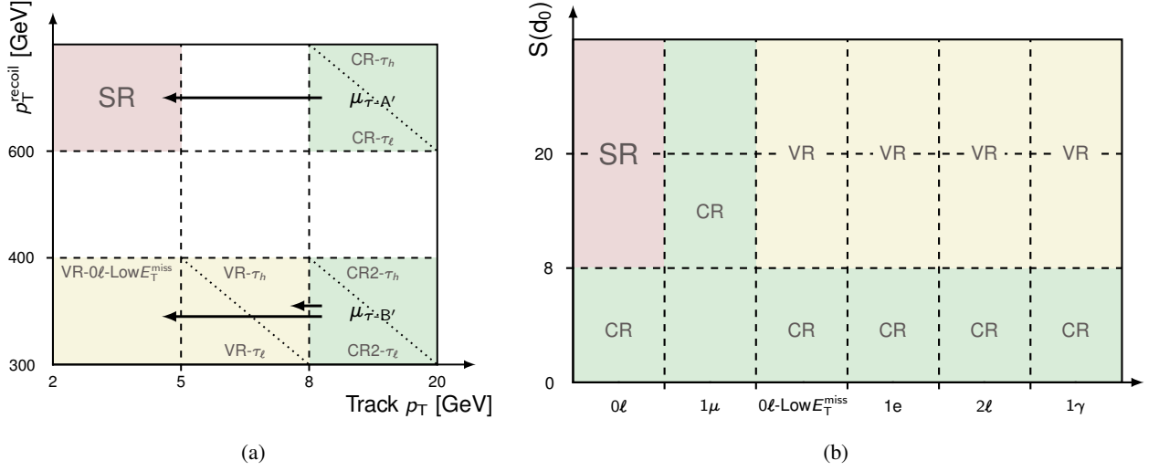
Figure 6: Schematics illustrating the selection of the CRs and VRs used to estimate (a) the tau track background and (b) the QCD track background, along with the orthogonality with respect to the SR. The arrows in (a) indicate the direction of extrapolation in the kinematic phase space which is validated in the VRs.
