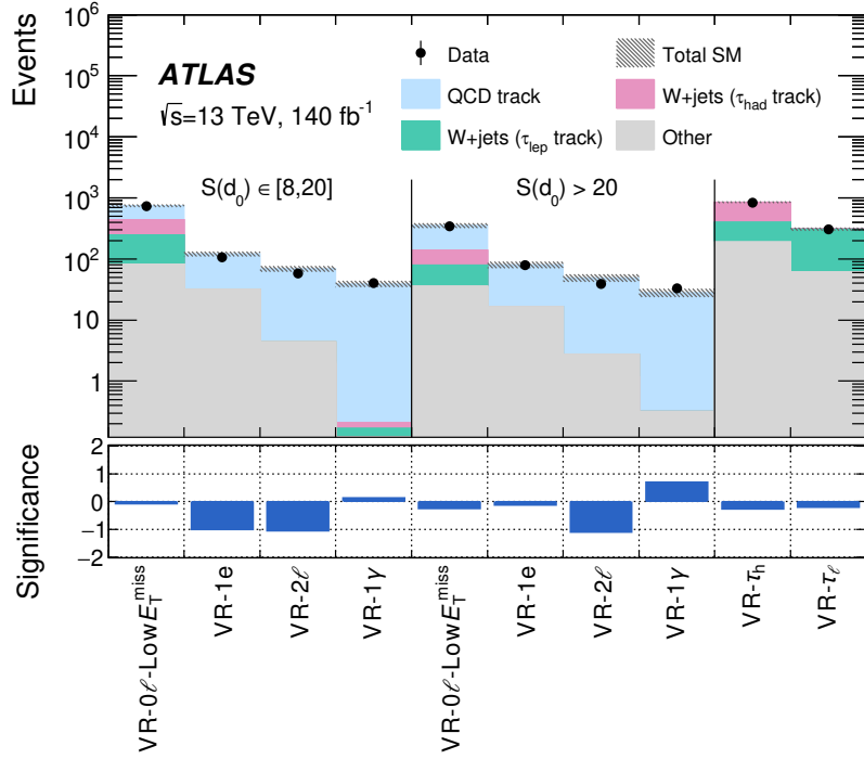
Figure 4: Comparisons of the observed data and the expected SM background in the VRs after the profile likelihood fit in the CRs. The hatched band indicates the total uncertainty on the SM background expectation, including both statistical and systematic uncertainties. The bottom panel shows the statistical significances [77] of the discrepancy between the expected and the observed event yields.
