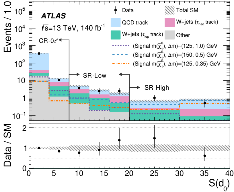
Figure 2: Postfit S(d_0) distribution in, and near, the SR and the adjacent control region CR-0 \ell . The selection criterion on the variable shown by each plot is removed, while the arrow indicates the cut value to define the region. The SM background expectation is shown as a histogram stack, and a few representative signal models are overlaid. The last bin includes the overflow. The hatched band indicates the uncertainty on the mean value of the SM background expectation, while the error bars on the black dots represent the Poisson error associated with the event yields.
