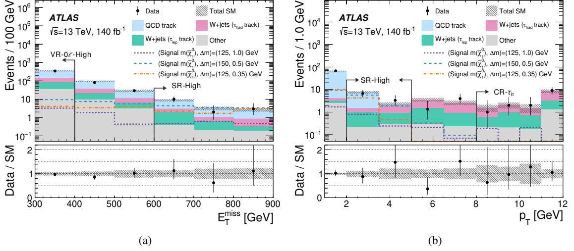
Figure 5: Distributions of E_T^{\text{miss}} and track p_T in, and near, the phase-space of SR-High. The selection criterion on the variable shown by each plot is removed, while the arrow indicates the cut value to define the region. The SM background expectation is shown as a histogram stack, and a few representative signal models are overlaid. The last bin includes the overflow. The hatched band indicates the uncertainty on the mean value of the SM background expectation, while the error bars on the black dots represent the Poisson error associated with the event yields.
