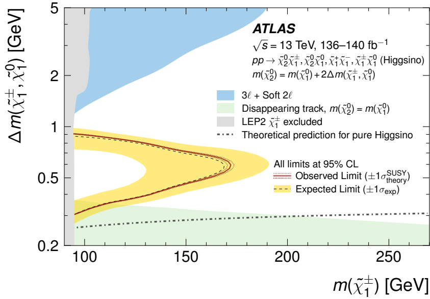
Figure 3: Expected (dashed black line) and observed (solid red line) 95% CL exclusion limits on the Higgsino simplified model being considered. These are shown with \pm 1\sigma_{\text{exp}} (yellow band) from experimental systematic and statistical uncertainties, and with \pm 1\sigma_{\text{theory}}^{\text{SUSY}} (red dotted lines) from signal cross section uncertainties, respectively. The limits set by the latest ATLAS searches using the soft lepton [19, 20] and disappearing track [16] signatures are illustrated by the blue and green regions, respectively, while the limit imposed by the LEP experiments [22] is shown in gray. The dot-dashed gray line indicates the predicted mass splitting for the pure Higgsino scenario [61].
