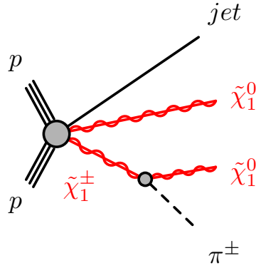
Figure 1: Example signal diagram for the targeted signature featuring a jet from initial-state radiation. For illustration, the \tilde{\chi}_1^\pm \tilde{\chi}_1^0 process is shown, while the production of \tilde{\chi}_1^+ \tilde{\chi}_1^- , \tilde{\chi}_1^\pm \tilde{\chi}_2^0 , and \tilde{\chi}_2^0 \tilde{\chi}_1^0 is considered in the search as well.
