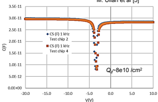
Fig. 6 Typical measurement of Flatband voltage with standard MOS capacitor [5].
