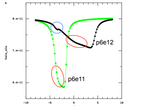
Fig. 9 TCAD simulations of Flatband voltage measurement with Ds of 6e12 and 6e11 /cm 2 under Qif of 1e11 /cm 2 and n-type charge traps in the p-layer region, together with the introduction of "setback" of p-layer to the metal area (blue circle).
