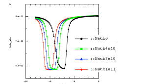
Fig. 10 TCAD simulations of Flatband voltage measurement with n-type surface contamination, under Ds of 6e11 /cm 2 , and n-type charge traps in the p-layer region.
