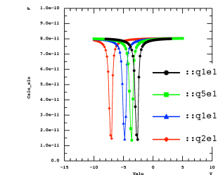
Fig. 7 TCAD simulations of Flatband voltage with Qif of 1e10, 5e10, 1e11, 2e11 /cm².
