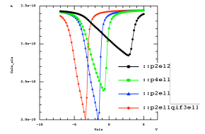
Fig. 8 TCAD simulations of Flatband voltage measurement with Ds of 2e12, 4e11, 2e11 /cm 2 under Qif of 1e11 /cm 2 . An extra is Ds of 2e11 (under Qif of 3e11 /cm 2 )
