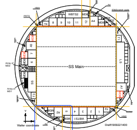
Fig. 1 Wafer layout of barrel sensor, Short-strip type (SS). QA chips are groups of test structures (encircled in blue), diced out in orange into Testchip&MD8 and Mini&MD8, one set per wafer.
