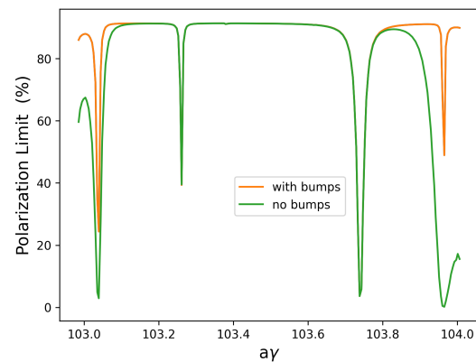
Figure 3: Polarization levels from first-order analytical \tau_{dep} with and without harmonic bumps optimized at 45.82 GeV ( a\gamma = 103.983 ) using the Rossmannith-Schmidt scheme in V22 lattice
