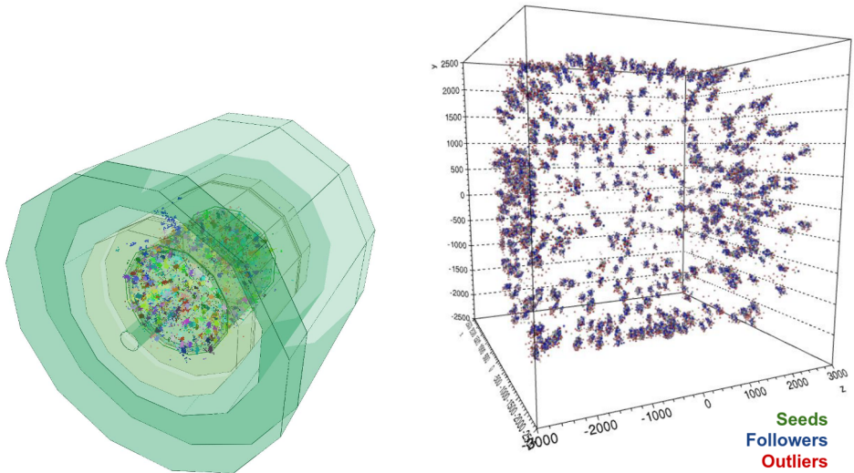
(a) Simulated photon clusters shown with CED (C-Event display, see Section 2.4). (b) Reconstructed clusters from CLUE.
