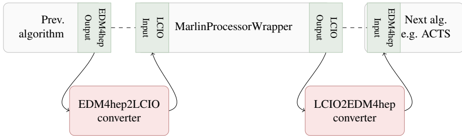
Figure 2: Schematic of how Marlin processors are integrated into Gaudi workflows in Key4hep.
