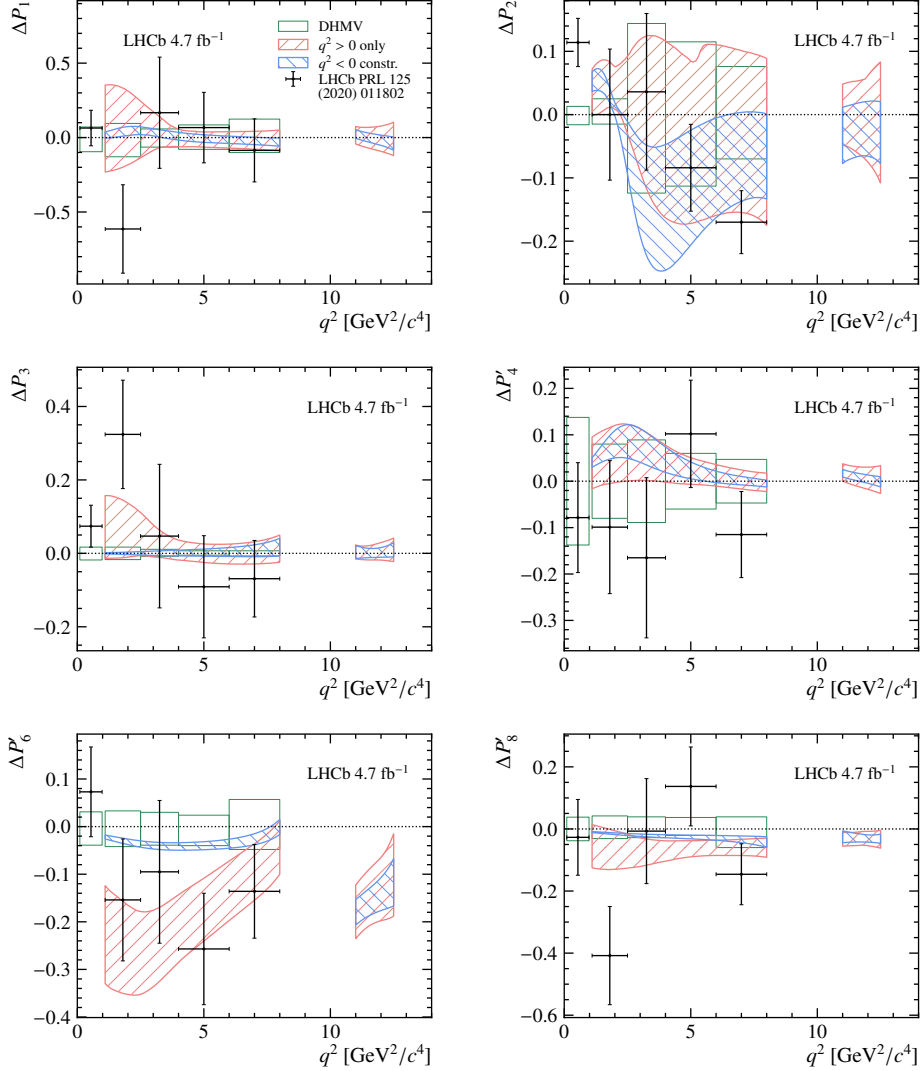
Figure 3: Non-local contributions to the angular observables (P-basis) obtained from data fits with (blue) and without (red) constraints from q^2 < 0 . The shaded regions are shown at 68% confidence level. When available, the difference between the LHCb binned angular analysis [10] and SM central-value from Refs. [33, 68] is overlaid for reference (black dots), together with the uncertainty on the SM prediction (green).
