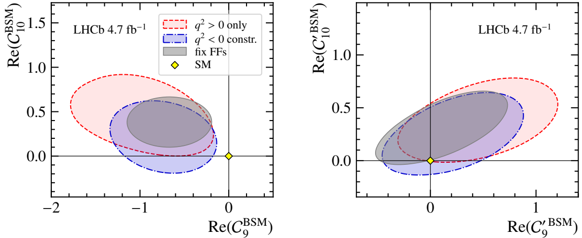
Figure 1: Two-dimensional profile-likelihood contours of the (left) C_9^{\text{BSM}}-C_{10}^{\text{BSM}} and (right) C_9'^{\text{BSM}}-C_{10}'^{\text{BSM}} pairs of Wilson coefficients at 68% confidence level with (blue) and without (red) SM constraints at q^2 < 0 . The fit is also repeated considering local FFs to be fixed to their SM predictions (grey) [16, 25, 31].
