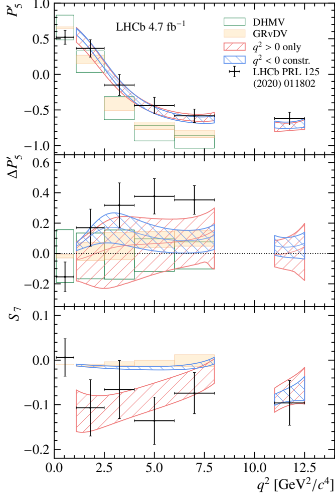
Figure 2: Determination of the (top) P'_5 and (bottom) S_7 angular observables obtained from the amplitude fit. Results are shown for fits with (blue) and without (red) constraints from q^2 < 0 , at 68% confidence level. The LHCb binned angular analysis [10] (black dots) and SM predictions from DHMV [33, 68] (green) and GRvDV [16, 25, 31] (yellow) are overlaid for reference. The center panel shows the non-local contributions to P'_5 determined from the amplitude fit. Here the difference between the LHCb binned angular analysis [10] and SM central-value from DHMV is overlaid for reference (black dots), together with the uncertainty on the DHMV SM prediction (green) and difference between the SM predictions from GRvDV and DHMV (yellow).
