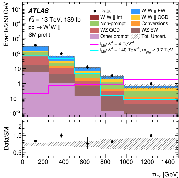
Figure 7: The observed m_{\ell\ell} distribution and the SM expectation. Data are shown as black markers with vertical error bars representing the statistical uncertainty. Filled histograms show contributions of SM processes, with the hatched error band corresponding to the total uncertainty. The sums of W^{\pm}W^{\pm}jj and W^{\pm}Zjj EFT contributions that correspond to the M0 operator with its Wilson coefficient set to its observed upper limit are shown as continuous lines for two cases, one where no unitarisation cut-off is applied, and another where the EFT contributions above m_{WV} > 0.7 \text{ TeV} are removed. Overflow events are included in the last bin. The lower panel shows the ratio of data to SM prediction.
