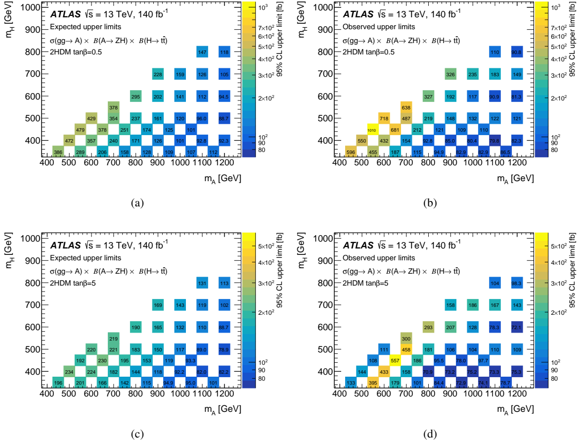
Figure 9: Expected and observed upper limits at 95% CL on \sigma(gg \rightarrow A) \times B(A \rightarrow ZH) \times B(H \rightarrow t\bar{t}) . The limits are shown for \tan\beta = 0.5 (a,b) and \tan\beta = 5 (c,d). The \tan\beta value is relevant only for the choice of A boson width.
