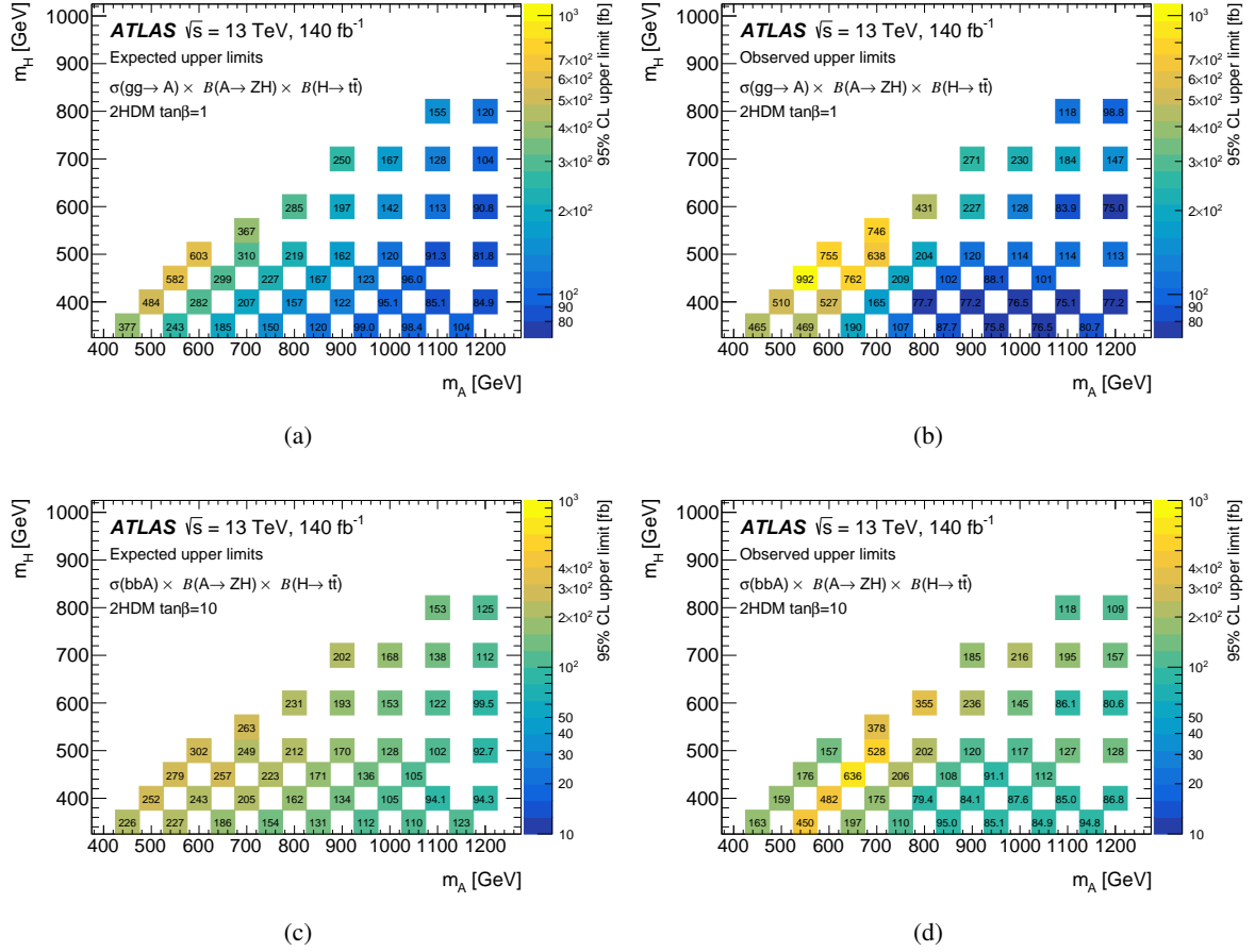
Figure 5: Expected (a,c) and observed (b,d) upper limits at 95% CL on \sigma(gg \rightarrow A) \times B(A \rightarrow ZH) \times B(H \rightarrow t\bar{t}) (a,b) and \sigma(bbA) \times B(A \rightarrow ZH) \times B(H \rightarrow t\bar{t}) (c,d) in the (m_A, m_H) plane. The limits are shown for either \tan\beta = 1 or \tan\beta = 10 in ggF or bbA production, respectively. The \tan\beta value is relevant only for the choice of A boson width.
