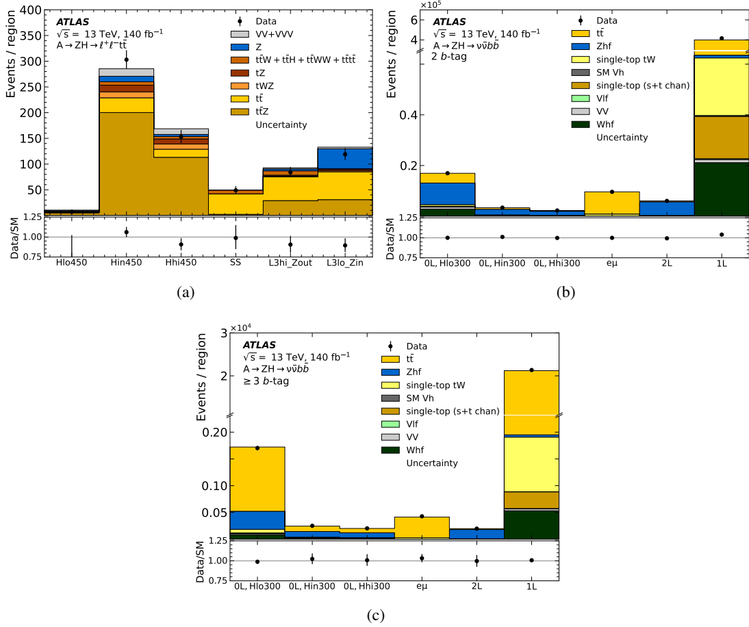
Figure 2: Yields in the SR, CRs and VRs used in the \ell^+\ell^-t\bar{t} channel (a) and in the 2- b -tag (b) and \geq 3 - b -tag (c) regions of the \nu b \bar{b} channel. The yields are obtained from a background-only fit to data. The region names are defined in Tables 2 and 3. The value next to the region name refers to the m_H hypothesis. The data are represented as black points and the associated error bars represent the statistical uncertainty. The background uncertainty (hashed band) shows the post-fit statistical and systematic components added in quadrature.
