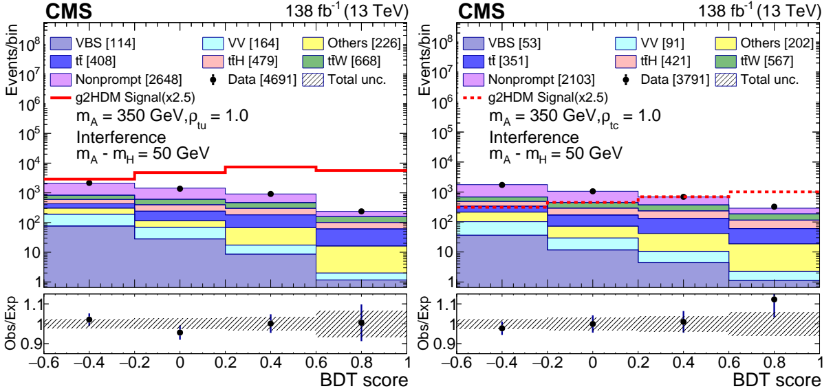
Figure 3: Post-fit distributions of the BDT discriminants combining the categories e^\pm e^\pm , \mu^\pm \mu^\pm , and e^\pm \mu^\pm , and all data-taking periods, for m_A = 350 GeV with \rho_{\text{tu}} = 1.0 (left), and \rho_{\text{tc}} = 1.0 (right) with the A-H interference. The numbers in square brackets represent the yields for each sample. The uncertainty bars on the points represent the statistical uncertainties in the data. Beneath each plot the ratio of data to predictions is shown. The uncertainty bars in the ratio plots include statistical uncertainties in the data and the total uncertainty in the background predictions, and the hatched bands represent the total uncertainty in the background predictions.
