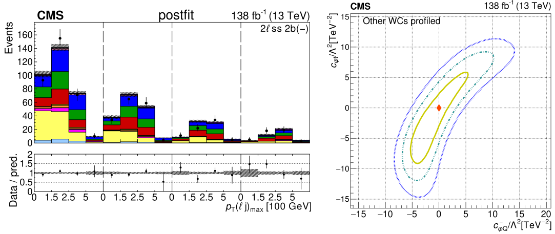
Figure 4: Post fit distribution of the variable p_T(lj)_{max} in bins of the jet multiplicity for a category of events containing two charged leptons with the same sign, a negative lepton charge sum and two hadronic b jets (left). Confidence contours from a two dimensional scan of c_{\phi t} and c_{\phi Q}^- while the remaining 24 WCs are profiled (right) [8].
