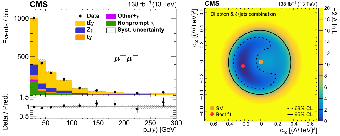
Figure 1: Post fit event yields as a function of the reconstructed photon p_T for the \mu^+\mu^- channel (left) [6]. Results from the two dimensional scan of the WCs c_{IZ} and c_{IZ}^I using the combination of the reconstructed photon p_T in the dilepton [6] and the \ell +jets [9] channels (right).
