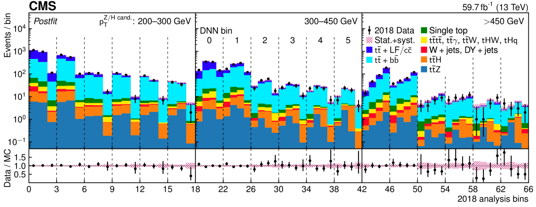
Figure 2: Post fit distribution of the large-radius jet ( Z/H candidate) invariant mass m_{SD} in bins of the DNN score and its p_T [7].
