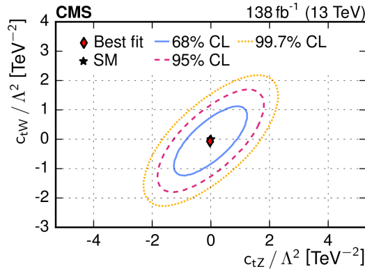
Figure 3: Two dimensional confidence contours of c_{tW} and c_{tZ} while having other WCs set to their SM value [7].
