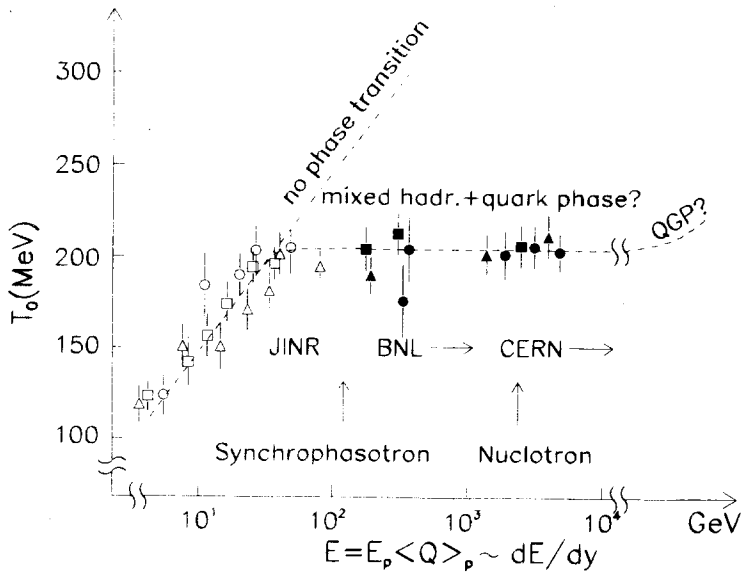
Figure 4: Inverse slope parameters T_0 versus E = E_p \langle Q \rangle_p \sim dE/dy : open circles, open triangles and open squares— K_S^0 , \Lambda and proton JINR data; black circles, black triangles and black squares— neutral (charged) kaons, \Lambda and proton data of BNL (17) and CERN (18). To make an adequate comparison, the T_0 parameters (not the Boltzmann temperatures T_B ) are shown on this figure, because T_B values are not given in CERN papers.
