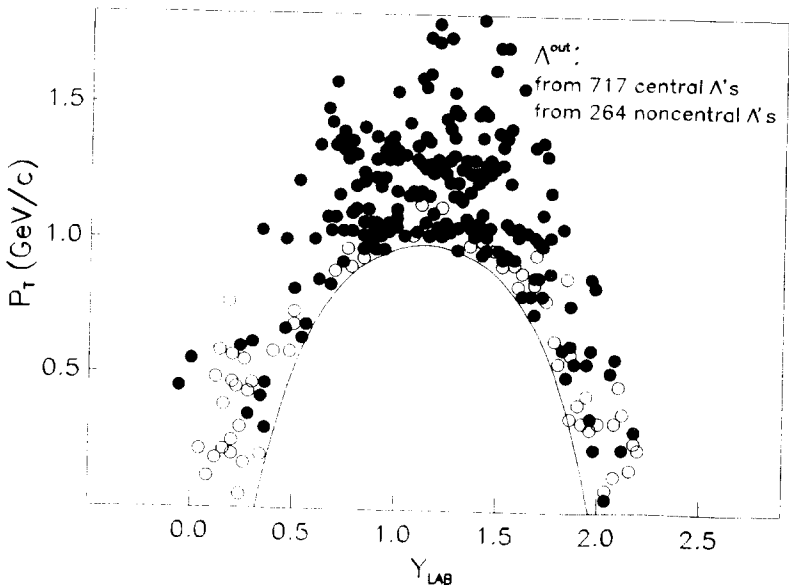
Figure 2: P_T - Y_L plot for commulative \Lambda hyperons produced: in non central HeLi CC-collisions selected from 264 \Lambda 's (open circles) and in central CNe, ONe, CCu, CZr, MgMg collisions from 717 \Lambda 's (black circles) at momenta 4.2 - 4.5 A GeV/c outside kinematical limits for NN interactions, outlined by solid lines
