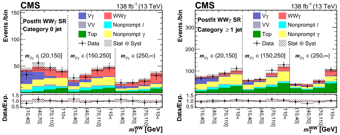
Figure 3: The unrolled two-dimensional m_T^{WW} - m_{\ell\ell\gamma} distributions in category 0 jet (left) and \geq 1 jet (right) after the fit to data. The data are compared with the sum of the signal and expected background. The black points with error bars represent the data and their statistical uncertainties, whereas the hatched bands represent the total uncertainties in the predictions.
