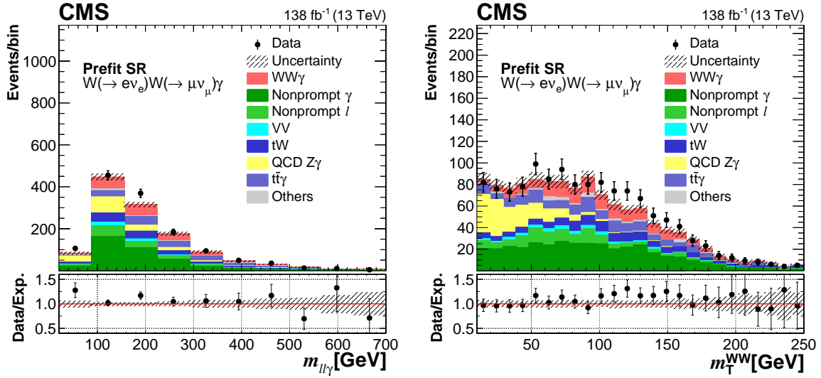
Figure 2: The distributions of the invariant mass of the dilepton-photon system (left) and the transverse mass of the WW system (right) after the signal region selection and before the fit to the data. The black points with error bars represent the data and their statistical uncertainties, whereas the shaded band represents the Monte Carlo statistical uncertainties.
