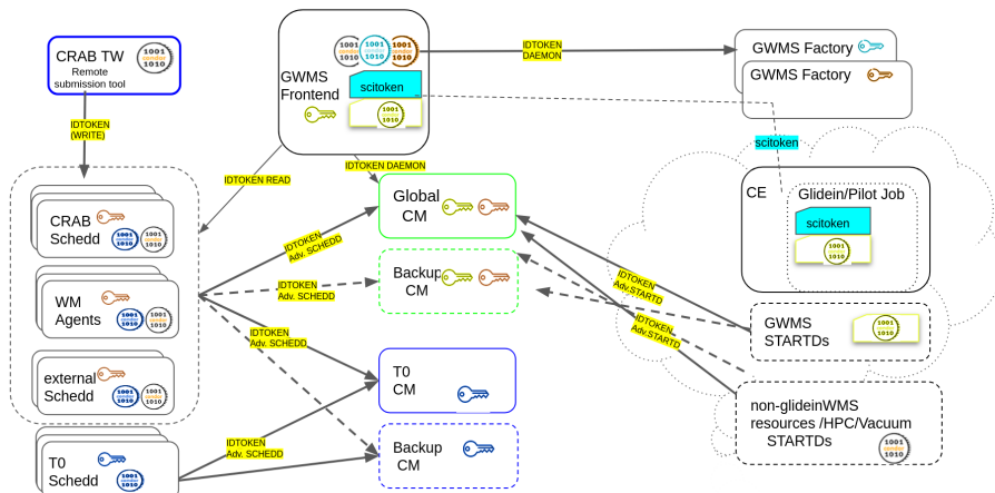
Figure 3. The CMS Global Pool components deployment, as described in section 2.
