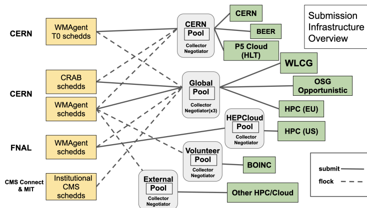
Figure 2. CMS SI current configuration, including multiple federated pools of resources aggregated from diverse providers (green boxes) and sets of distributed job schedders, handling the Tier-0 and centralized production workloads (WMAgent), as well as analysis job submission (CRAB).
