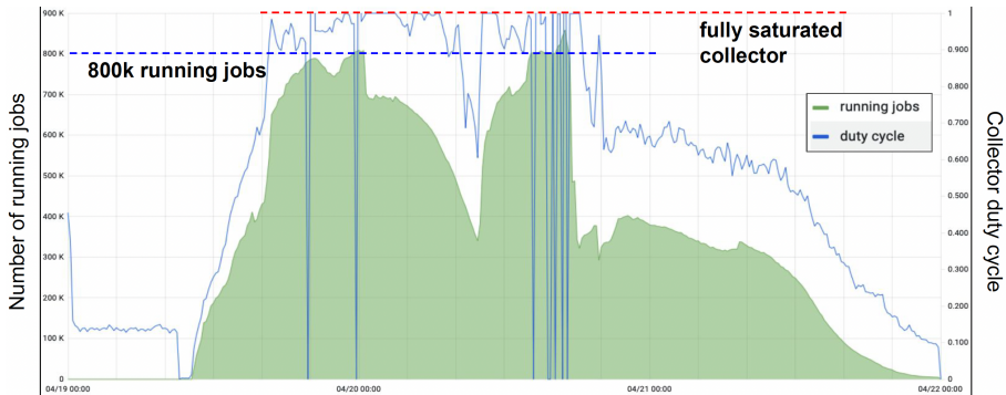
Figure 5. Final results of the Spring 2023 scalability tests of the CMS HTCondor Global Pool, reaching the simultaneous execution of approximately 800k jobs.
