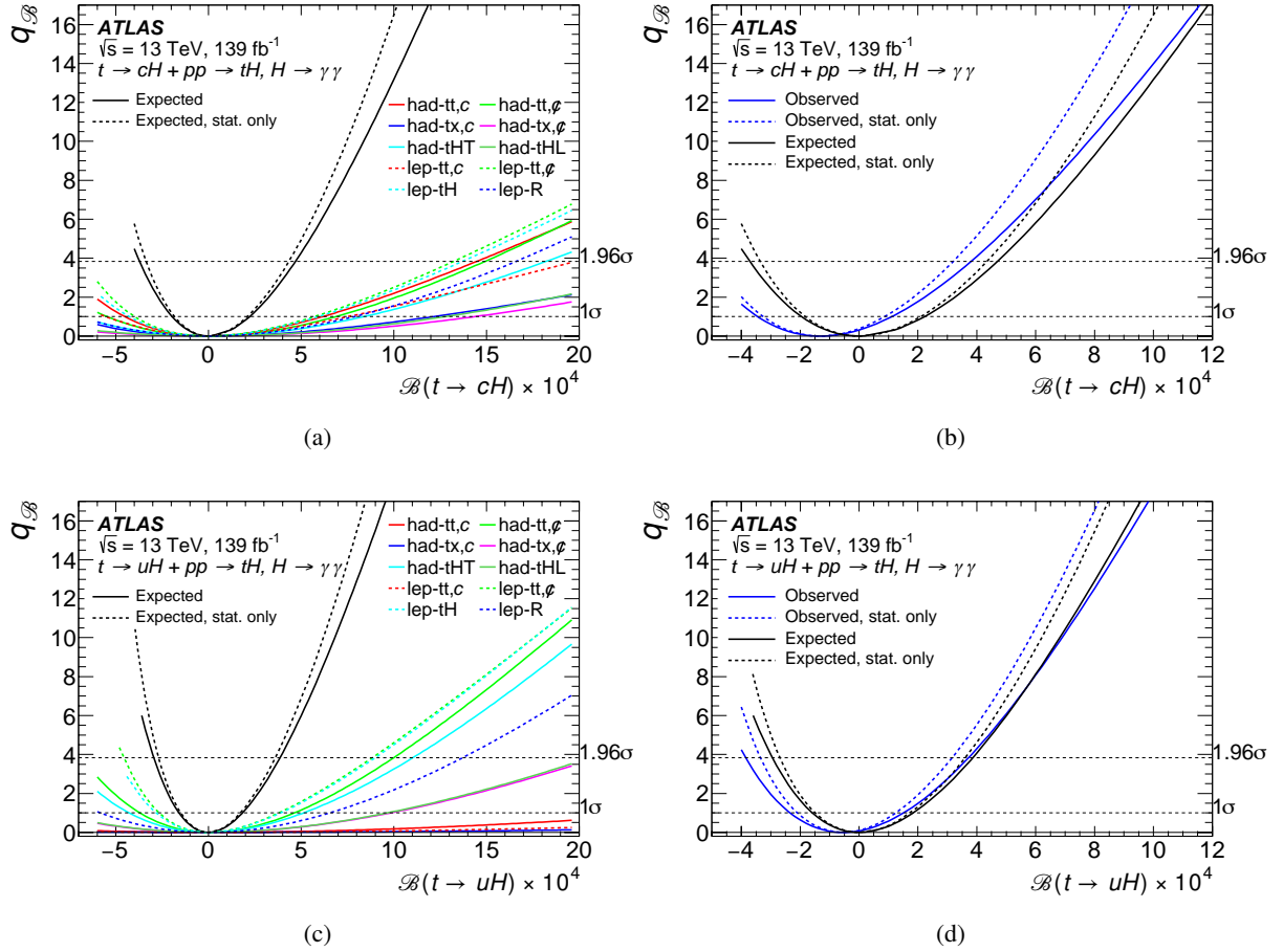
Figure 9: Evolution of q_{\mathcal{B}} , the negative log-profile-likelihood ratio (times 2), as a function of the t \rightarrow cH (top) and t \rightarrow uH (bottom) branching ratios. In (a) and (c) the evolutions for each category and the combined sample are shown for the expected result in the absence of signal, while (b) and (d) show a comparison between the observed result and the expectation in the absence of signal. The likelihood functions are only defined for a positive expected number of events, hence some categories and combined curves do not cover the full scanned range.
