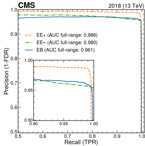
Figure 14: Precision (1-FDR) versus Recall (TPR) curve for the zero-occupancy scenario after spatial and time corrections are applied. The inset plot shows a zoomed-in view. The full-range area under the curves (AUC) are also indicated.
