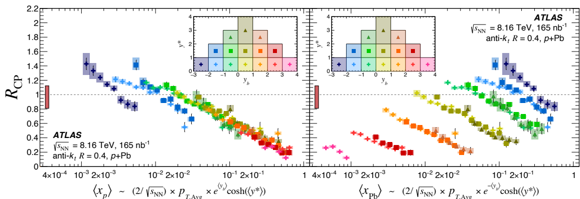
Figure 1: R_{CP} plotted as a function of approximated x_p (left panel) and x_{pb} (right panel), constructed using \langle y_b \rangle and \langle y^* \rangle . An inset legend is included, showing the (y_b, y^*) bins, and their corresponding markers. The proton-going direction is defined by y_b > 0 . Shaded rectangles represent the total systematic uncertainty, while the vertical error bars represent the statistical uncertainty. The solid rectangle on the left-side of each panel represents the uncertainty on the T_{AB} .
