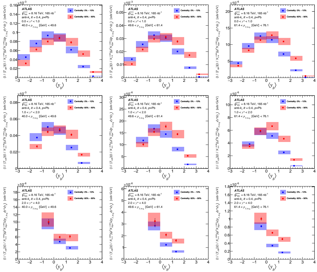
Figure 4: \langle T_{\text{AB}} \rangle normalized per-event dijet yields in 0–10% (blue) and 60–90% (red) collisions as a function of \langle y_b \rangle in three representative p_{T,\text{Avg}} bins for 0.0 < y^* < 1.0 (top row), 1.0 < y^* < 2.0 (middle row), 2.0 < y^* < 4.0 (bottom row). Shaded rectangles represent the total systematic uncertainty, while the vertical error bars represent the statistical uncertainty. The systematic uncertainties for the two distributions are highly correlated.
