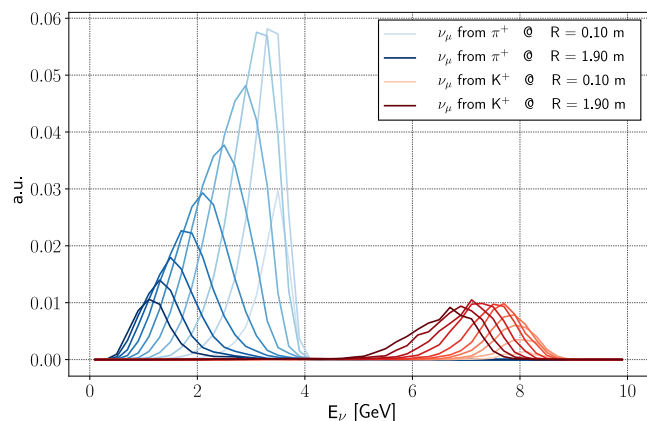
Fig. 29 Energy distributions of \nu_\mu events from the decay tunnel at different detector radii. Each distribution represents a \pm 10 cm radius interval around its central value.
