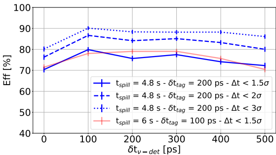
Fig. 33 Efficiency of tagging a \nu_e - e^+ pair from the same K_{e3} as a function of the neutrino detector resolution. An extraction spill of 4.8 s and a t_0 layer time resolution of \delta t_{tag}=200 ps (blue lines) are considered. The effect of a 1.5\sigma (solid-line), 2\sigma (dashed-line) and 3\sigma (dotted-line) cut around the peak is also reported. As a comparison, the efficiency corresponding to an extraction spill of 6 s, a \delta t_{tag}=100 ps and a 1.5\sigma cut around the peak is also shown (red line).
