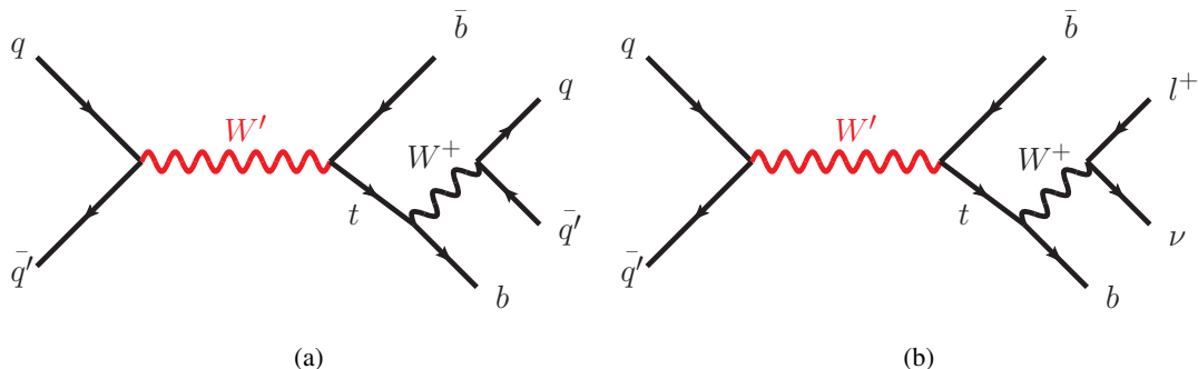
Figure 1: Representative leading-order Feynman diagrams for s -channel W' -boson production with decay into tb , for (a) a top quark decaying into a W boson that decays hadronically (all-hadronic decay mode) and (b) a top quark decaying into a W boson that decays into a lepton and neutrino (lepton+jets decay mode).
