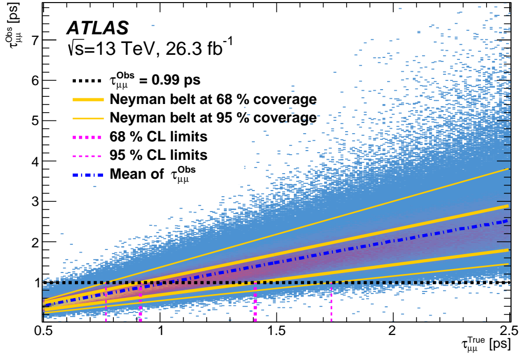
Figure 4: 68% and 95% CL bands obtained with a Neyman construction based on MC pseudo-experiments for the signal and background components. The yellow lines interpolate the band boundaries in order to smooth the effects of limited number of MC pseudo-experiments used. The dashed-dotted blue line corresponds to the average expected \tau_{\mu\mu}^{\text{Obs}} value at a given \tau_{\mu\mu}^{\text{True}} value. The horizontal dashed black line corresponds to the experimentally observed value of \tau_{\mu\mu}^{\text{Obs}} = 0.99 ps, yielding a 68% CL band of [0.92, 1.41] ps (thick vertical dashed purple lines) and a 95% CL band of [0.77, 1.73] ps (thin vertical dashed purple lines). The same construction at the \tau_{\mu\mu}^{\text{Obs}} corresponding to \tau_{\mu\mu}^{\text{True}} = \tau_{\mu\mu}^{\text{SM}} yields [1.44, 2.26] ps as 68% CL band.
