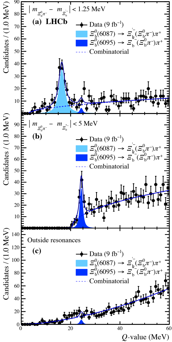
Figure 5: Distributions of the mass difference Q = m_{\Xi_b^0 \pi^+ \pi^-} - m_{\Xi_b^-} - 2m_\pi for selected \Xi_b^0 \pi^+ \pi^- candidates, (a) in the \Xi_b'^- mass window, (b) in the \Xi_b^{*-} mass window and (c) outside the mass windows of the intermediate resonances. The results of the simultaneous fit are superimposed.
