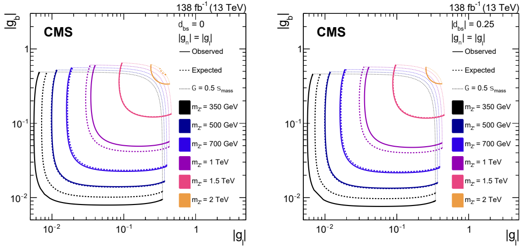
Figure 6: Observed (solid) and median expected (dashed) exclusion limits at 95% CL in the |g_b| - |g_l| plane for the LFU model. The scenarios considered have |d_{bs}| values of either 0 (left) or 0.25 (right). In all cases, we assume |g_\nu| = |g_l| . The exclusion limits are given up to coupling values at which the Z' width is equal to half of the \mu\mu invariant mass resolution, marked by the dotted curves. Beyond these coupling values, the narrow width approximation intrinsic to the search strategy is not considered valid. The enclosed regions are excluded.
