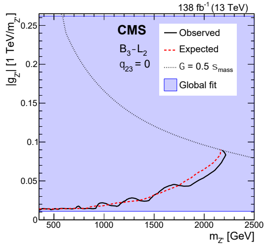
Figure 8: Exclusion limits at 95% CL in the |g_{Z'}|-m_{Z'} plane for the B_3-L_2 model [9] for a fixed value of \theta_{23} = 0 . The solid black (dashed red) curve represents the observed (median expected) exclusion. The dotted curve denotes the coupling values at which the Z' width equals one half of the \mu\mu invariant mass resolution. For larger values of the couplings, the narrow width approximation intrinsic to the search strategy is not considered valid. The region enclosed between the solid black (dashed red) and the dotted curves is (expected to be) excluded. The shaded blue area represents the |g_{Z'}| range preferred from the global fit in Ref. [9] at 95% CL.
