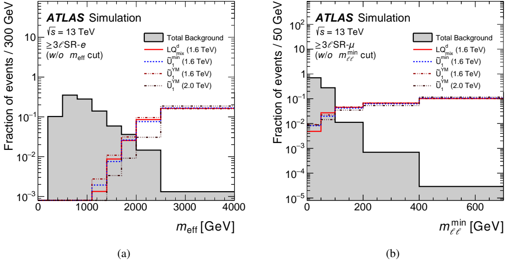
Figure 2: Comparison of the distribution of (a) m_{\text{eff}} in 3\ell\text{SR-}e or 4\ell\text{SR-}e region without an m_{\text{eff}} requirement, and (b) m_{\ell\ell}^{\min} in 3\ell\text{SR-}\mu or 4\ell\text{SR-}\mu region without a m_{\ell\ell}^{\min} requirement, between the total background (shaded histogram) and the various LQ signals. The shapes of these variables ( m_{\text{eff}} and m_{\ell\ell}^{\min} ) are very similar in the electron and muon channels. The last bin in each distribution contains the overflow.
