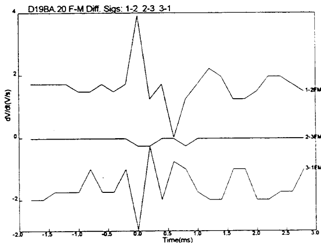
Fig. 4. Fast-Motion: Axial localization is visible from the difference signals of coils #1 (feed-end), #2 (middle), and #3 (return-end). Signal 2-3 is quiet, while 1-2 is a rough inverse of 3-1. Hence, the signal-source is within region #1.
