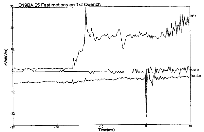
Fig. 6. 1st quench (#24): The largest fast-motion transient produced the stop-trigger ( t = 0 ) but occurred 17 ms after quench-initiation (BIFs @ t = -17 ms.). A smaller one was coincident with quench onset.
