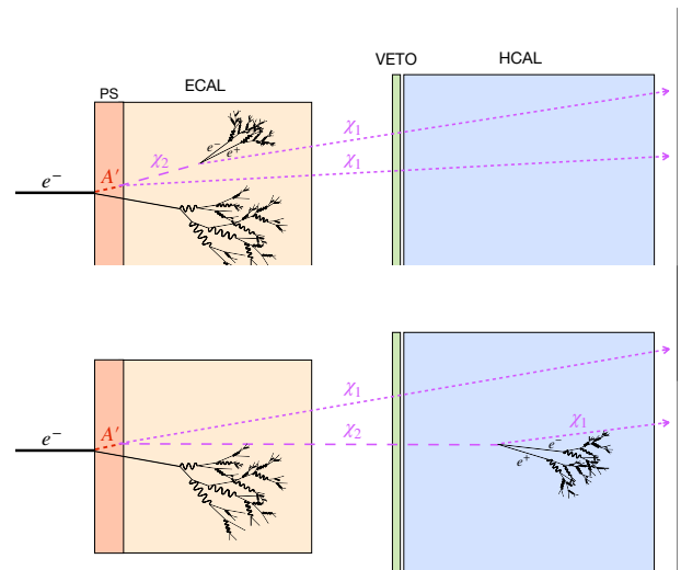
Fig. 3.1 Sketch of a semi-visible event in the NA64 setup. Note that only the detectors relevant for the discussion are depicted. The first drawing represents a prompt \chi_2 decay in the target, while in the second, \chi_2 has a longer lifetime and produces a leptonic pair in the HCAL.
