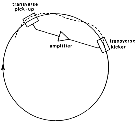
Fig. 2 Cooling of the horizontal betatron oscillation of a single particle.
