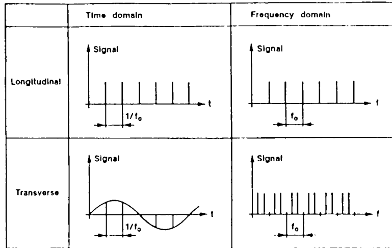
Fig. 4 Schottky signals in time domain and frequency domain.
