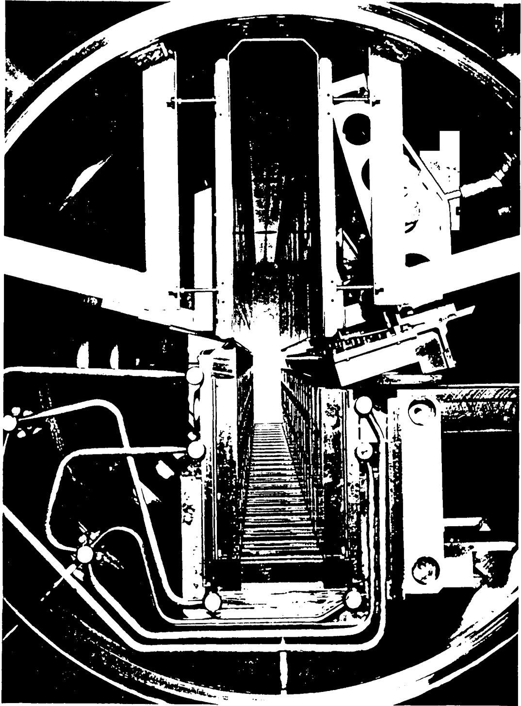
Fig. 12 Inside of a vacuum tank with precooled kickers at the left and space for the stack at the right. The ferrite frames of the kickers are open in the centre of the picture; they can be closed by the ferrite slabs mounted on the shutter that rotates around a pivot at the far right. Water tubes for cooling the ferrite may be seen.
