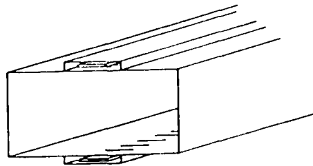
Fig. 9 Loop-type and ferrite ring-type pick-ups (or kickers). Note that for loop-type kickers the beam direction should be inverted.
