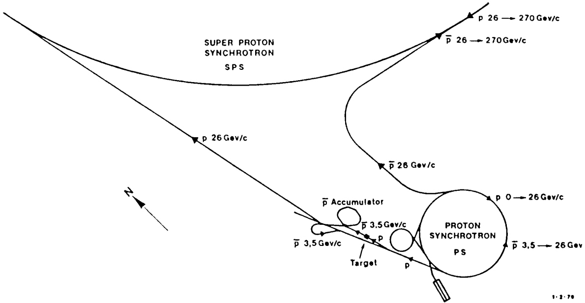
Fig. 1 Overall layout of the p-p̄ project.
