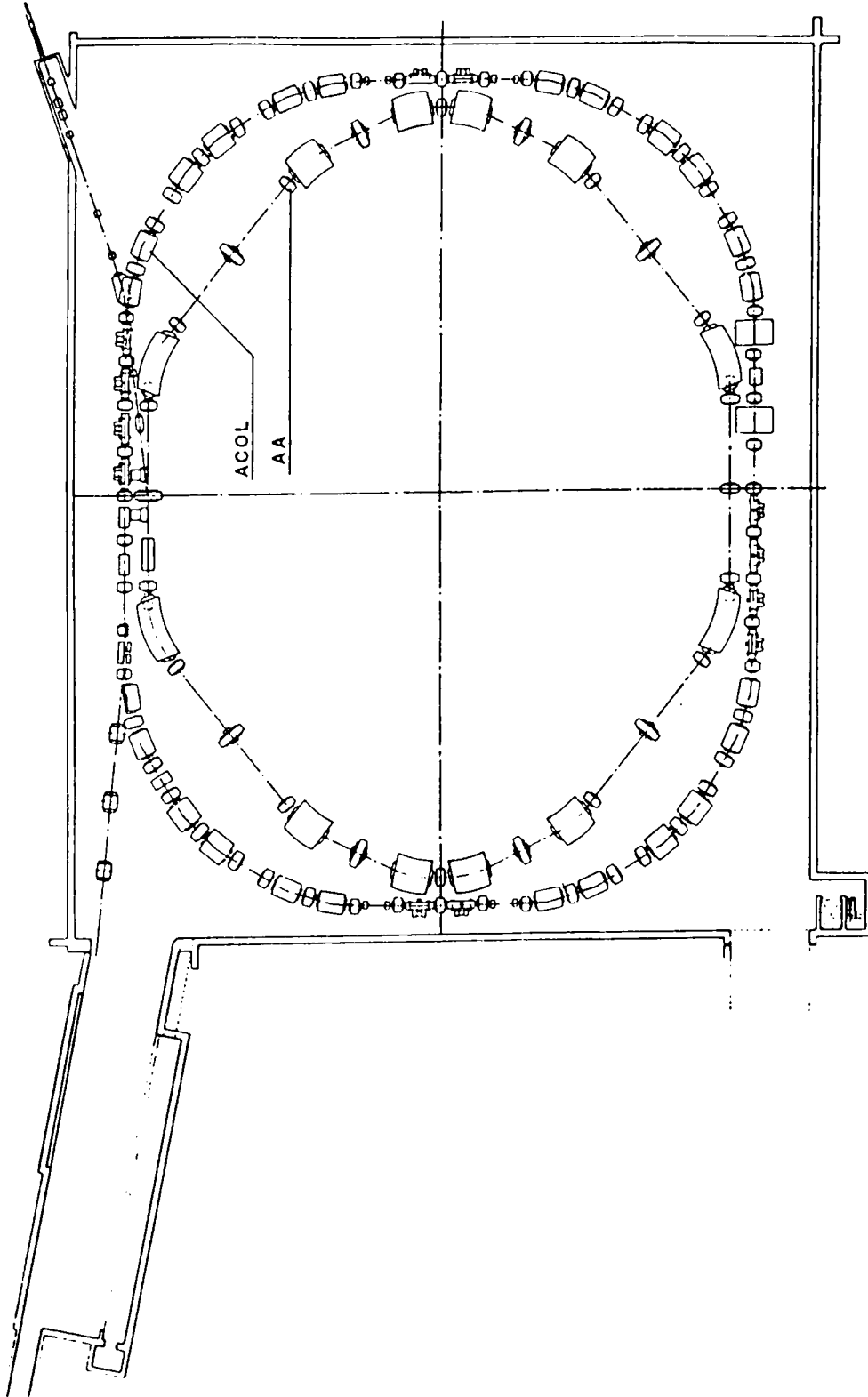
Fig. 16 The new ACOL ring (under construction) around the AA. This ring will increase the stacking rate by an order of magnitude. The stack will still be kept in the AA ring
